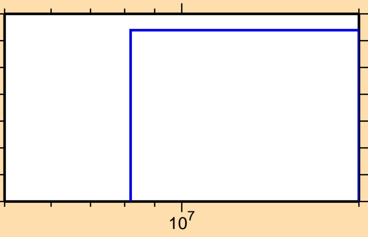
\sigma vs. E for ^{18}\text{F}(n,2n)
