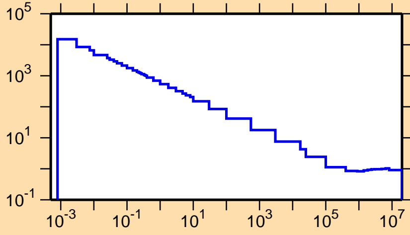
\sigma vs. E for ^{18}\text{F}(n,\text{nonel.})
