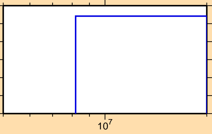
\sigma vs. E for ^{18}\text{F}(n,\text{He3})
