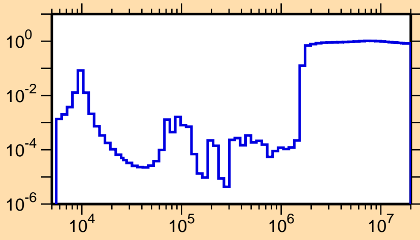
\sigma vs. E for ^{20}\text{F}(n,\text{nonel.})
