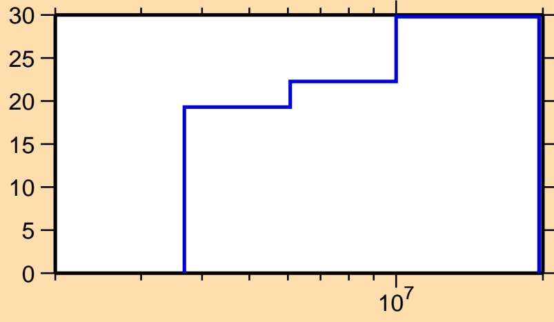
\Delta\sigma/\sigma vs. E for ^{20}\text{F}(n,n\text{cont.})
