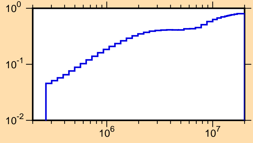
\mu vs. E for ^{22}\text{F}(\text{mt251})
