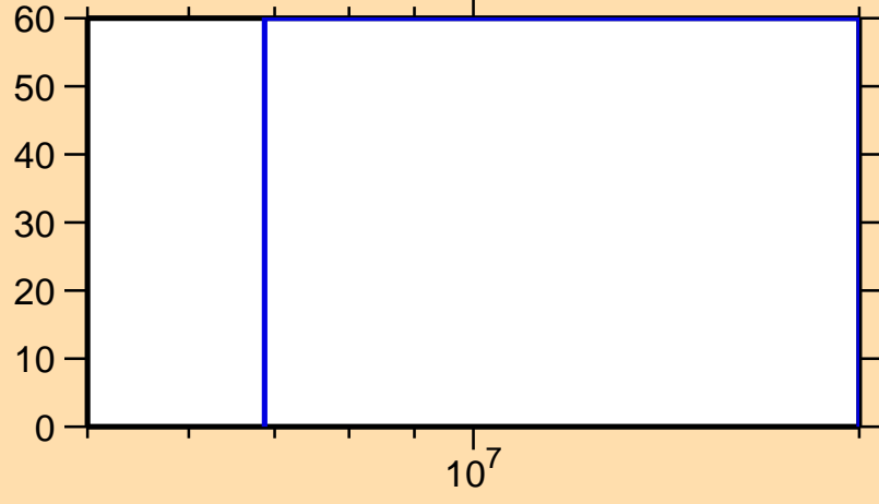
\Delta\sigma/\sigma vs. E for ^{22}\text{F}(n,n\text{cont.})
