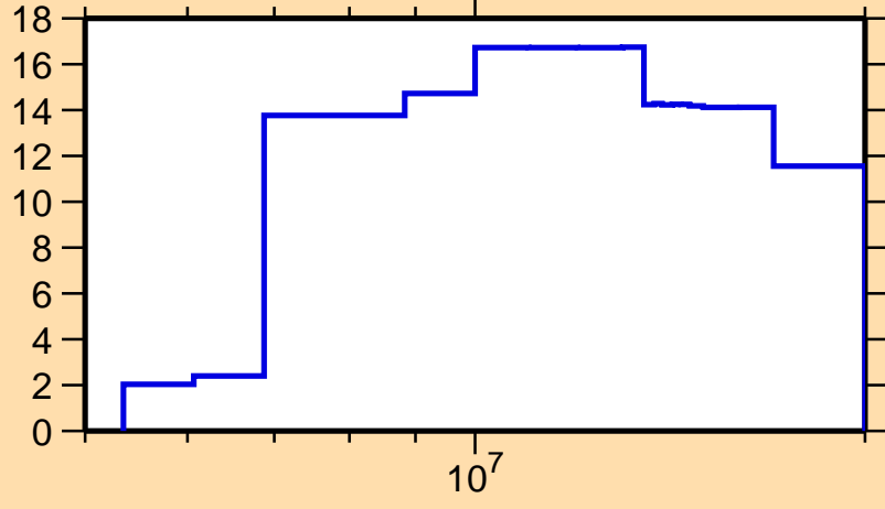
\Delta\sigma/\sigma vs. E for ^{22}\text{F}(n,el.)
