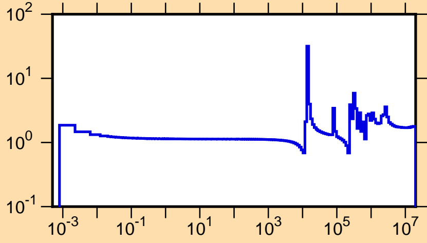
\sigma vs. E for ^{22}\text{F}(n,\text{tot.})
