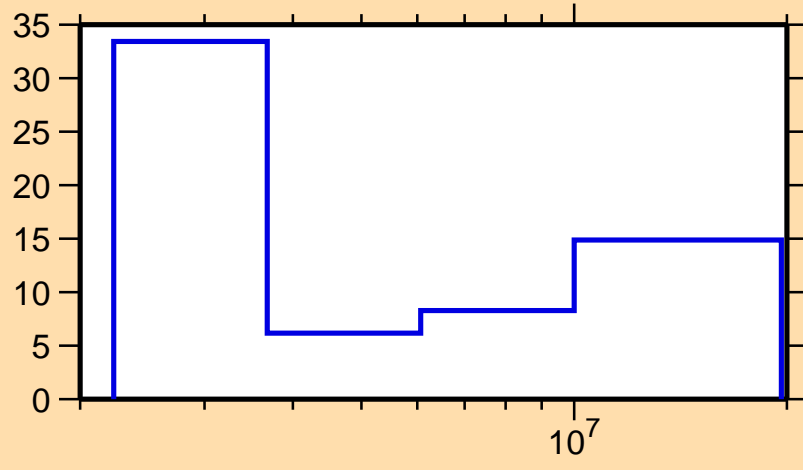
\Delta\sigma/\sigma vs. E for ^{22}\text{F}(n,\text{el.})
