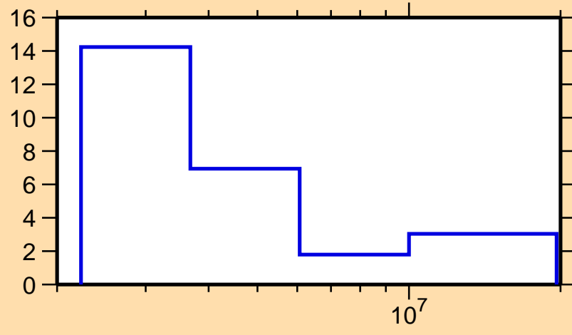
\Delta\sigma/\sigma vs. E for ^{22}\text{F}(n,\text{tot.})
