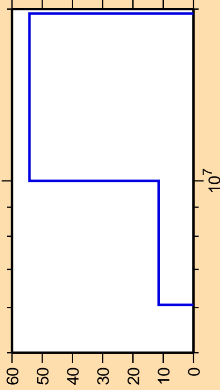
\Delta\sigma/\sigma vs. E for ^{22}\text{F}(n,n_1)
