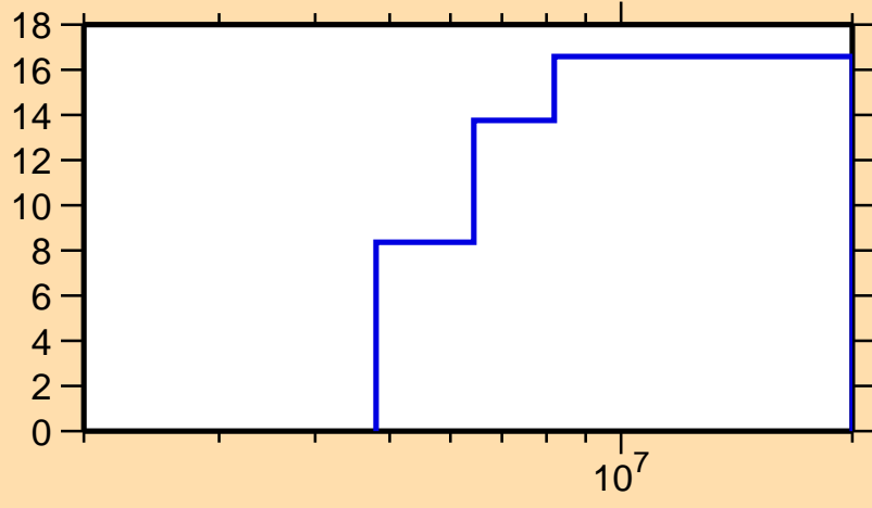
\Delta\sigma/\sigma vs. E for ^{22}\text{F}(n,n_1)
