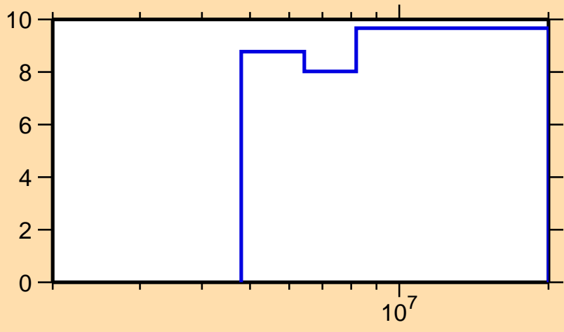
\Delta\sigma/\sigma vs. E for ^{22}\text{F}(n,\text{nonel.})
