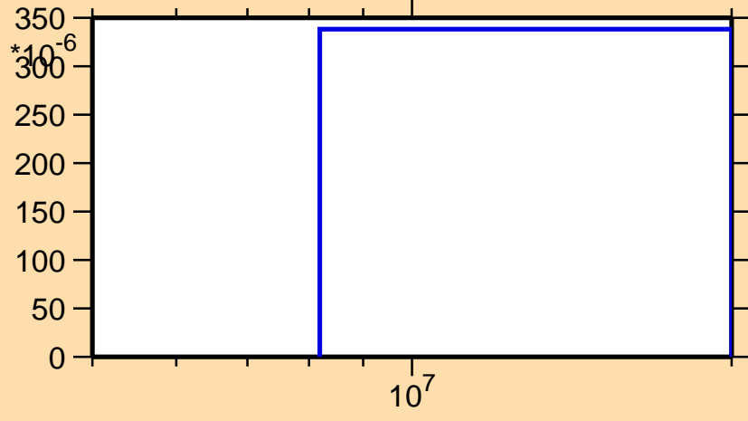
\sigma vs. E for ^{22}\text{F}(n,np)
