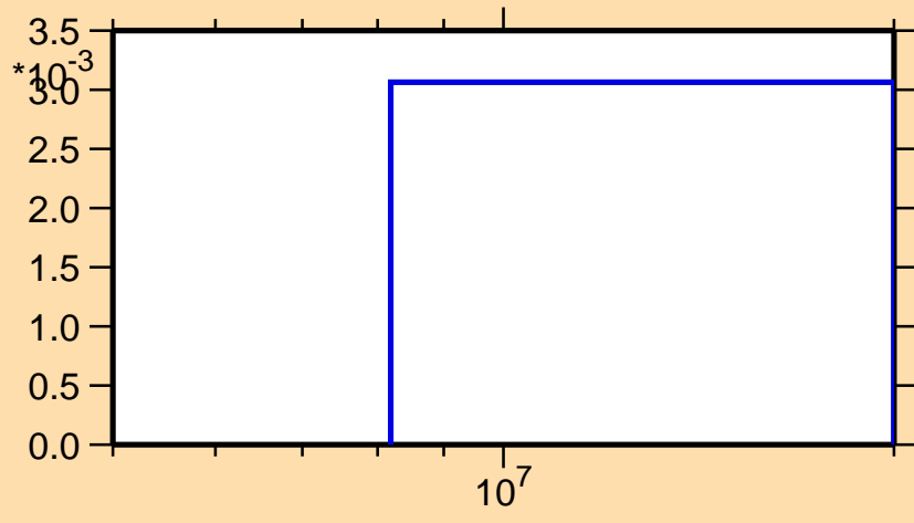
\sigma vs. E for ^{22}\text{F}(n,d)
