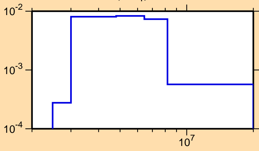
\sigma vs. E for ^{22}\text{F}(n,n_1)
