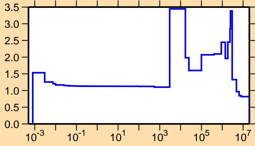
\sigma vs. E for ^{22}\text{F}(n,\text{el.})
