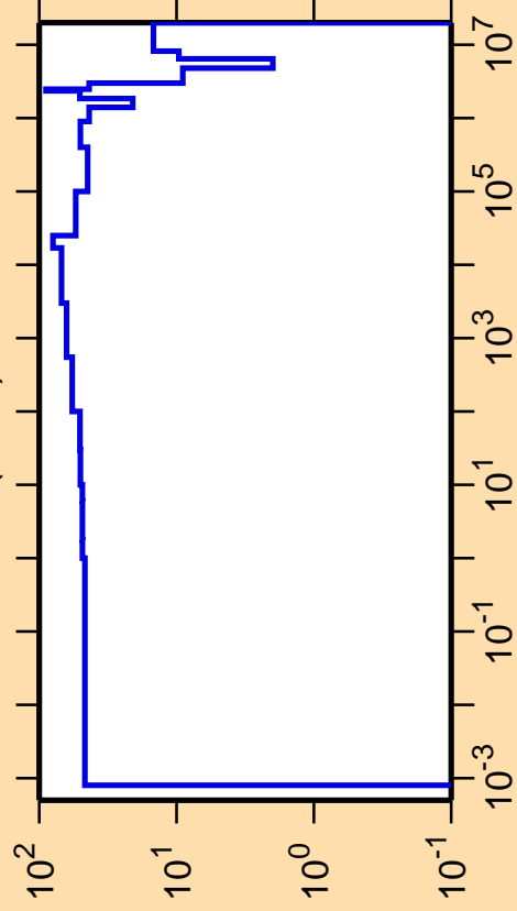
\Delta\sigma/\sigma vs. E for ^{22}\text{F}(n,\text{el.})
