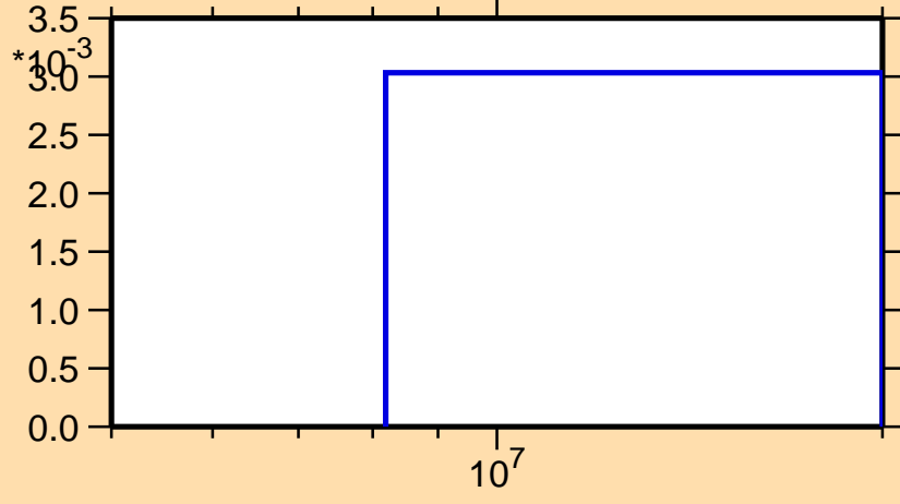
\sigma vs. E for ^{22}\text{F}(n,3n)
