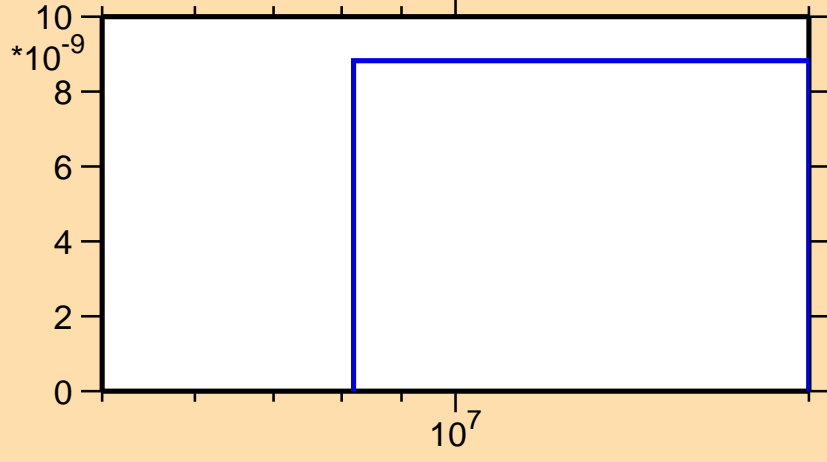
\sigma vs. E for ^{22}\text{F}(n,2n\alpha)
