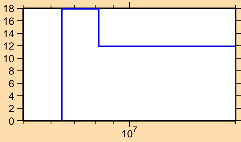
\Delta\sigma/\sigma vs. E for ^{22}\text{F}(n,2n)
