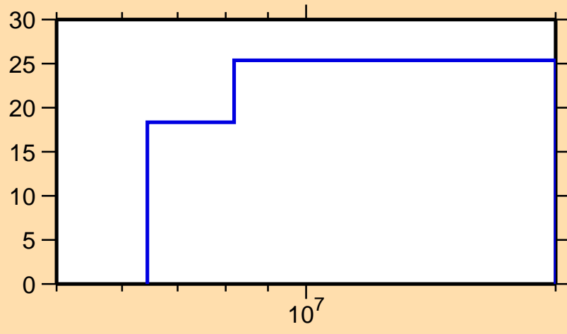
\Delta\sigma/\sigma vs. E for ^{22}\text{F}(n,\text{inel.})
