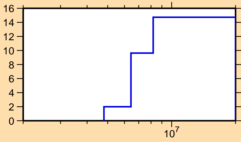
\Delta\sigma/\sigma vs. E for ^{22}\text{F}(n,el.)
