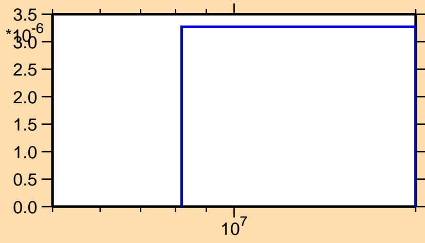
\sigma vs. E for ^{22}\text{F}(n,nd)
