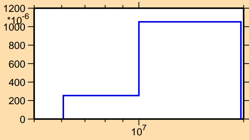
\sigma vs. E for ^{23}\text{F}(n,n\text{cont.})
