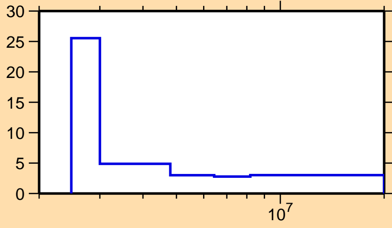
\Delta\sigma/\sigma vs. E for ^{23}\text{F}(n,\text{tot.})
