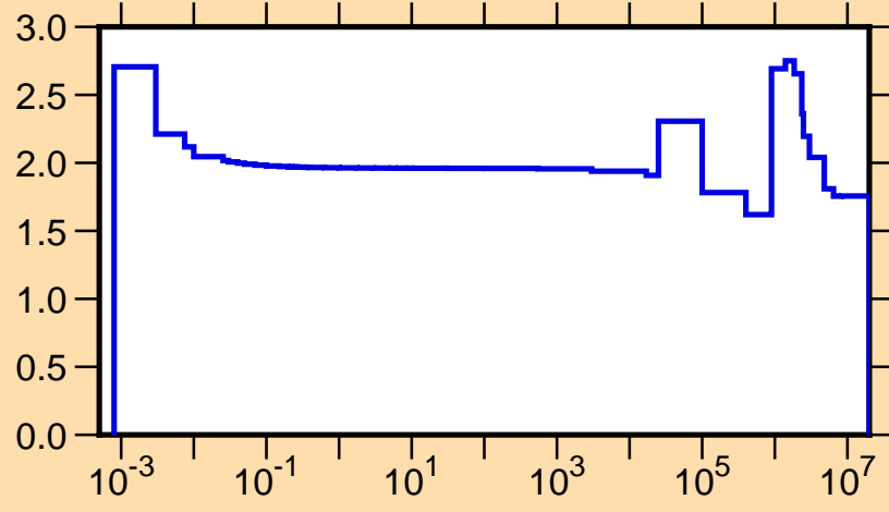
\sigma vs. E for ^{23}\text{F}(n,\text{tot.})
