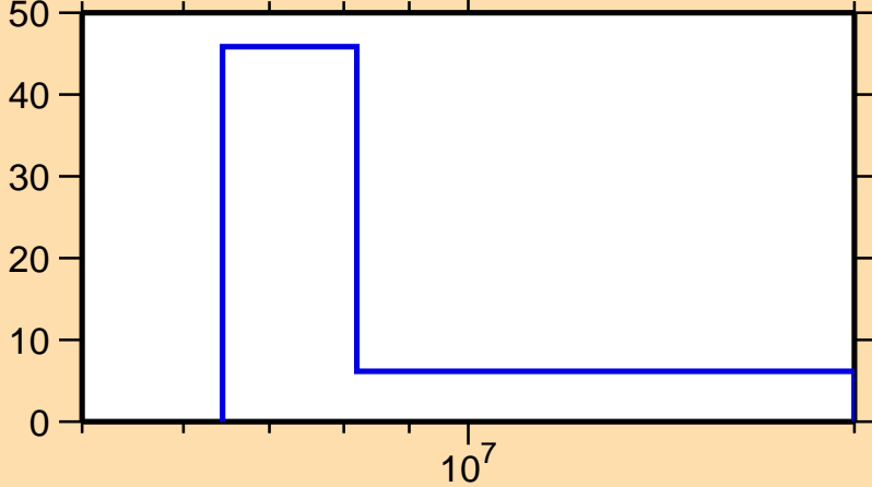
\Delta\sigma/\sigma vs. E for ^{23}\text{F}(n,2n)
