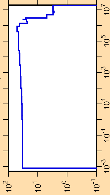
\Delta\sigma/\sigma vs. E for ^{23}\text{F}(n,\text{tot.})
