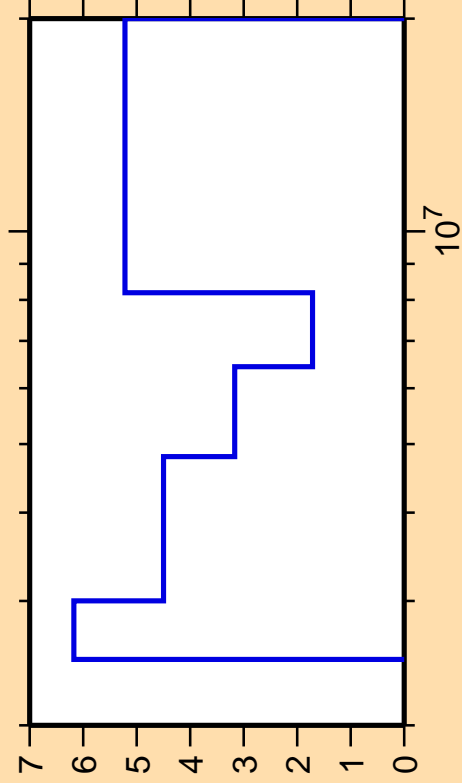
\Delta\sigma/\sigma vs. E for ^{23}\text{F}(n,\text{inel.})
