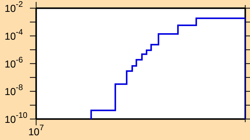
\sigma vs. E for ^{52}\text{Fe}(n,\text{pd})
