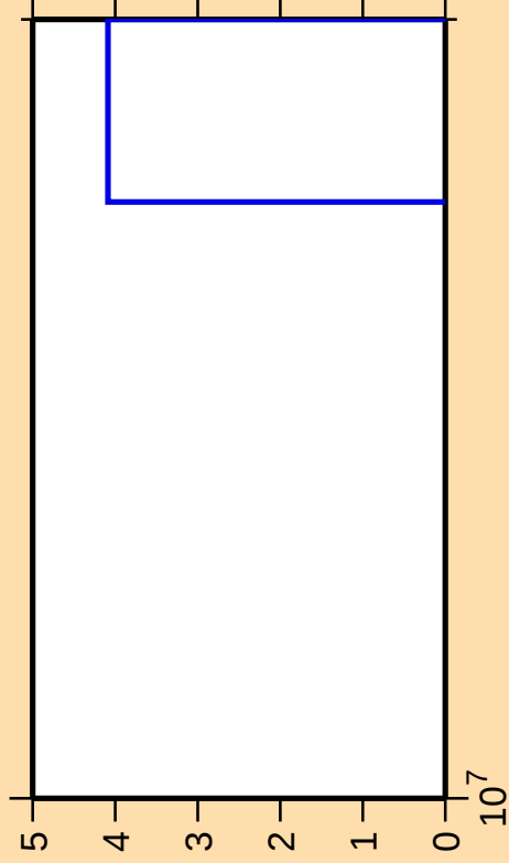
\Delta\sigma/\sigma vs. E for ^{52}\text{Fe}(\text{n},\text{pt})
