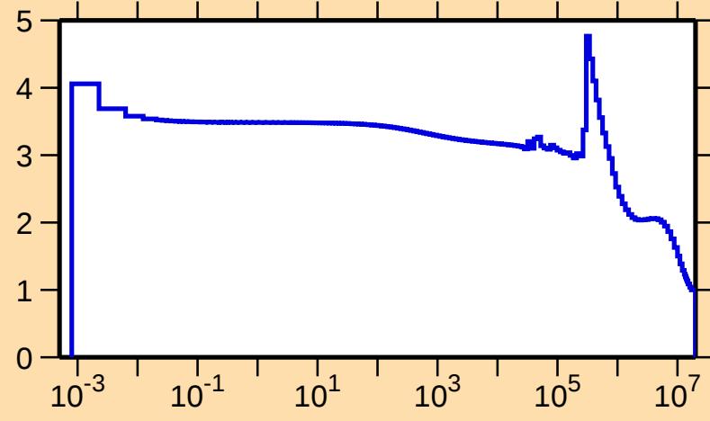
\sigma vs. E for ^{52}\text{Fe}(n,\text{el.})
