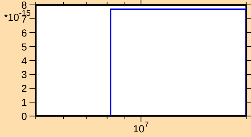
\sigma vs. E for ^{52}\text{Fe}(\text{n},\text{pt})
