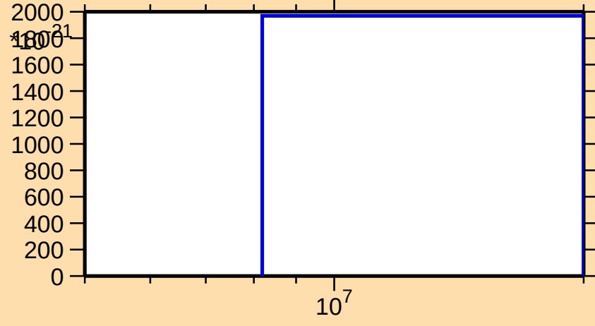
\sigma vs. E for ^{52}\text{Fe}(n,\text{nd})
