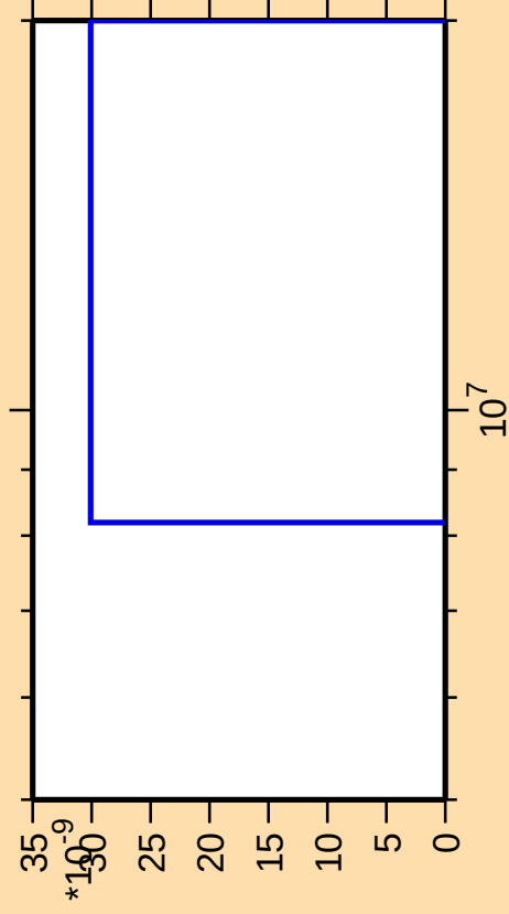
\Delta\sigma/\sigma vs. E for ^{52}\text{Fe}(\text{mt } 34)
