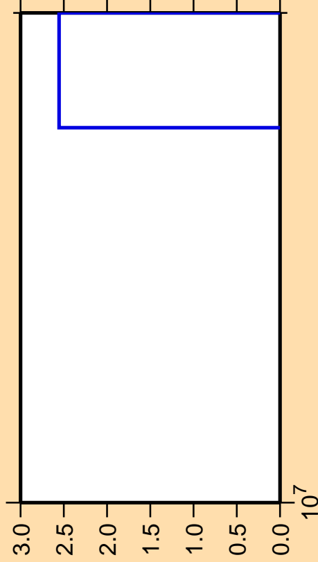
\Delta\sigma/\sigma vs. E for ^{52}\text{Fe}(n,nt)
