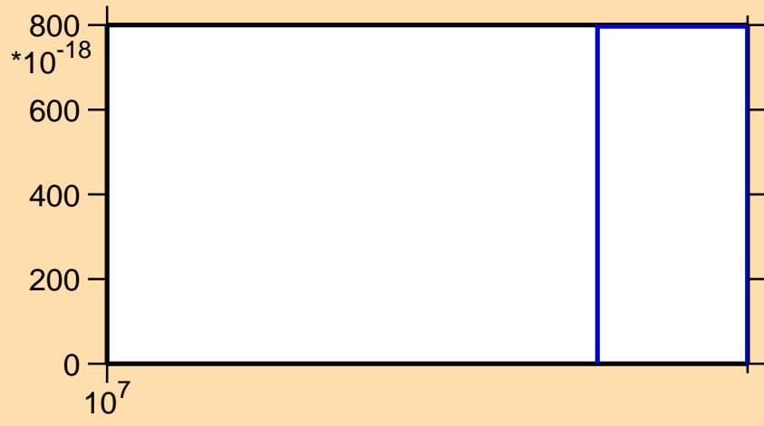
\sigma vs. E for ^{52}\text{Fe}(n,nt)
