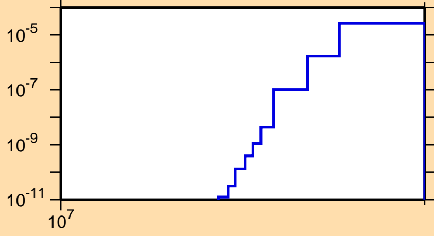
\sigma vs. E for ^{52}\text{Fe} (mt 45)
