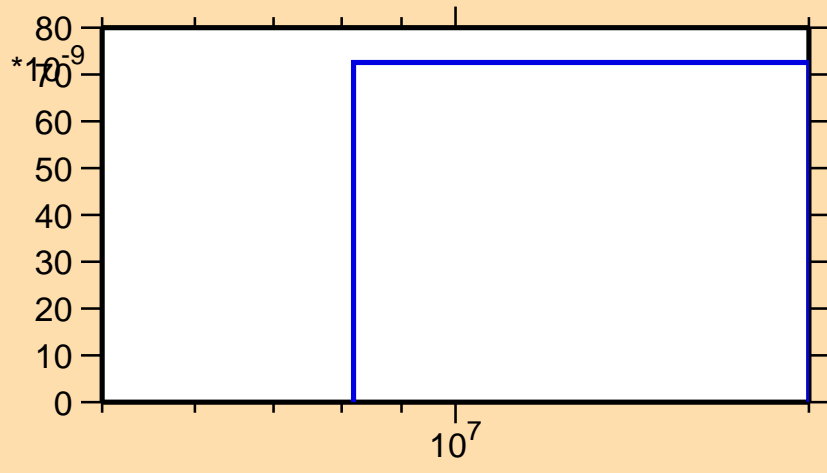
\sigma vs. E for ^{52}\text{Fe} (mt 34)
