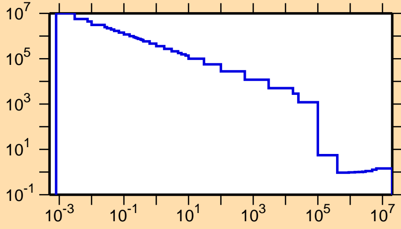
\sigma vs. E for ^{52}\text{Fe}(n,\text{nonel.})
