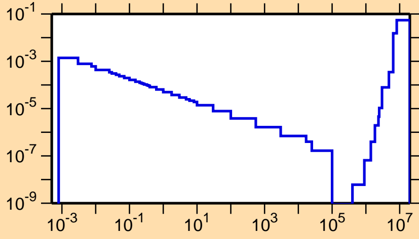
\sigma vs. E for ^{52}\text{Fe}(n,d)
