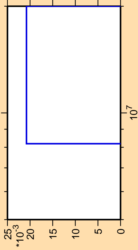
\Delta\sigma/\sigma vs. E for ^{52}\text{Fe}(n,nt)
