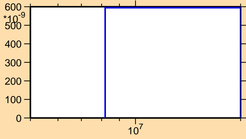
\sigma vs. E for ^{52}\text{Fe}(n,2np)
