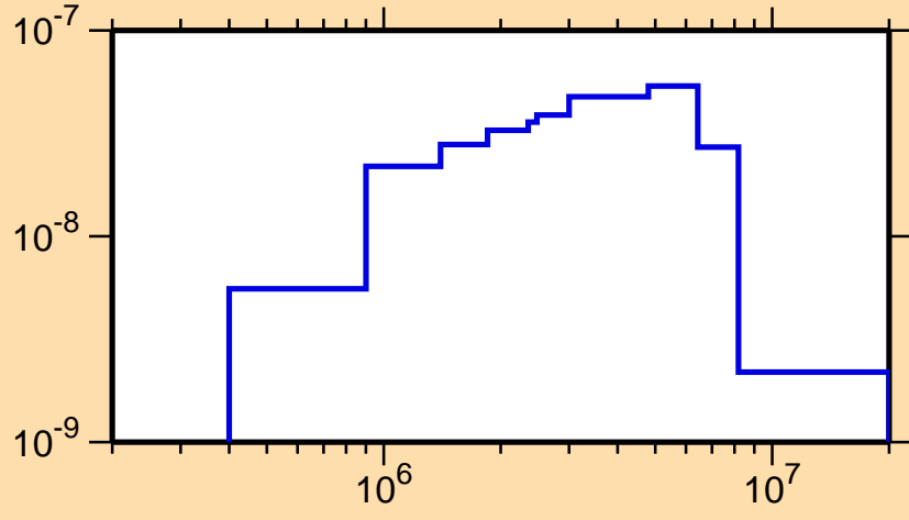
\sigma vs. E for ^{52}\text{Fe}(n,n_1)
