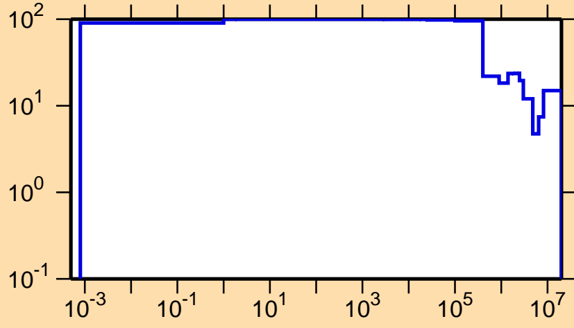
\Delta\sigma/\sigma vs. E for ^{52}\text{Fe}(n,el.)
