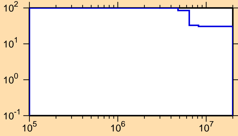
\Delta\sigma/\sigma vs. E for ^{52}\text{Fe}(n,ncont.)
