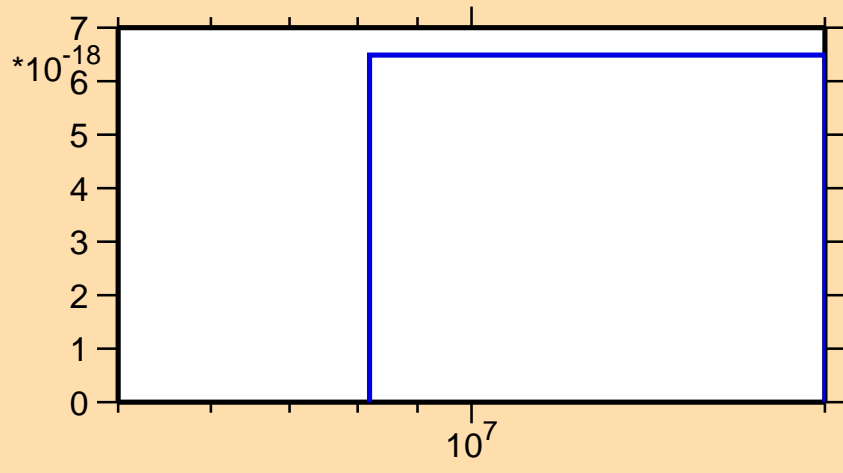
\sigma vs. E for ^{52}\text{Fe}(n,nt)
