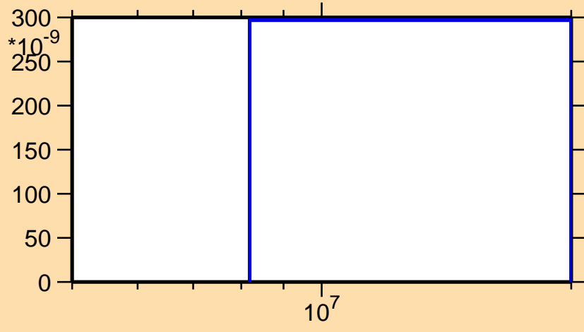
\sigma vs. E for ^{52}\text{Fe} (mt 45)
