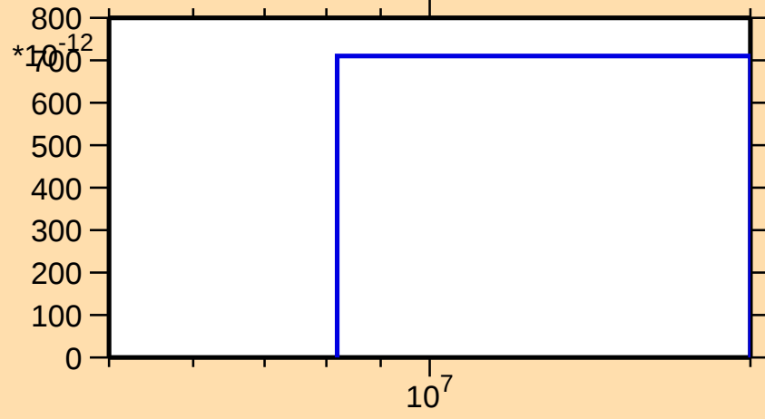
\sigma vs. E for ^{53}\text{Fe}(\text{n},\text{pt})
