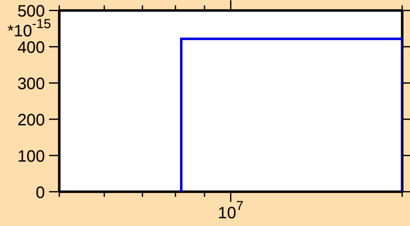
\sigma vs. E for ^{53}\text{Fe}(\text{mt } 34)
