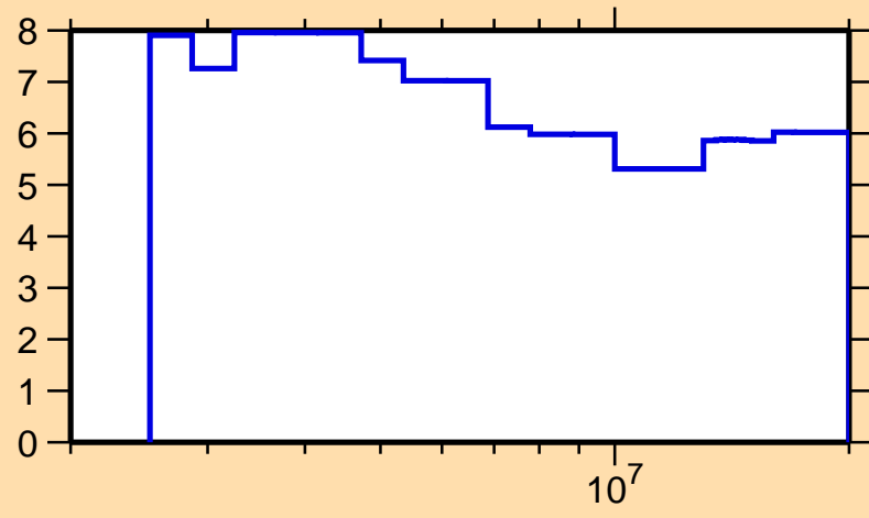
\Delta\sigma/\sigma vs. E for ^{57}\text{Fe}(n,n\text{onel.})
