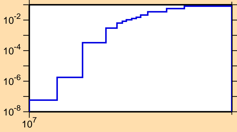
\sigma vs. E for ^{57}\text{Fe}(n,np)
