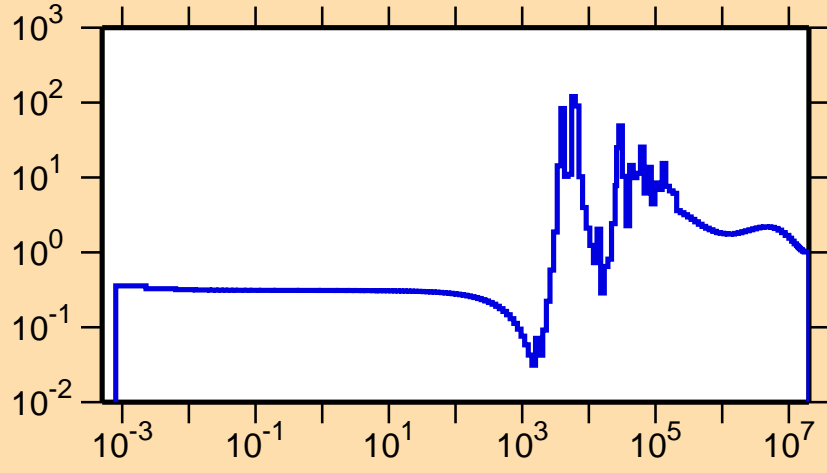
\sigma vs. E for ^{57}\text{Fe}(n,\text{el.})
