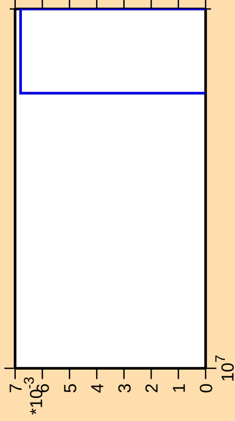
\Delta\sigma/\sigma vs. E for ^{60}\text{Fe}(n,\text{nt})
