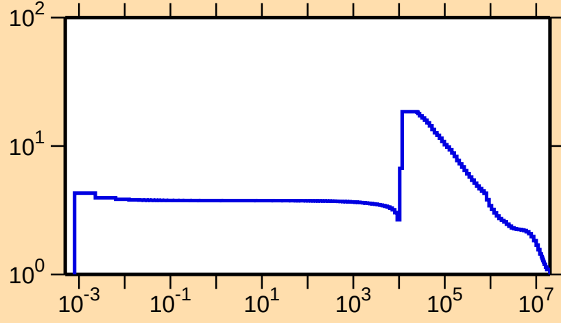
\sigma vs. E for ^{60}\text{Fe}(\text{n},\text{el.})
