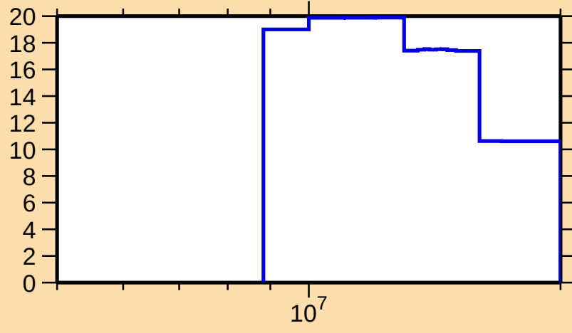
\Delta\sigma/\sigma vs. E for ^{60}\text{Fe}(n,\text{el.})
