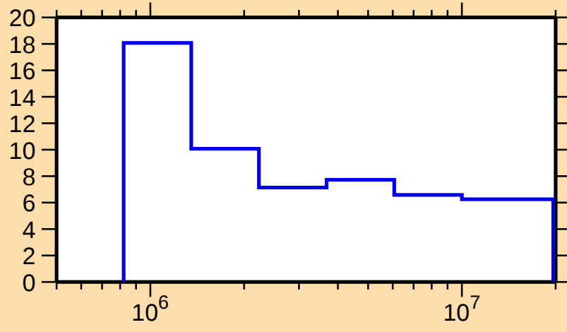
\Delta\sigma/\sigma vs. E for ^{60}\text{Fe}(\text{n,nonel.})
