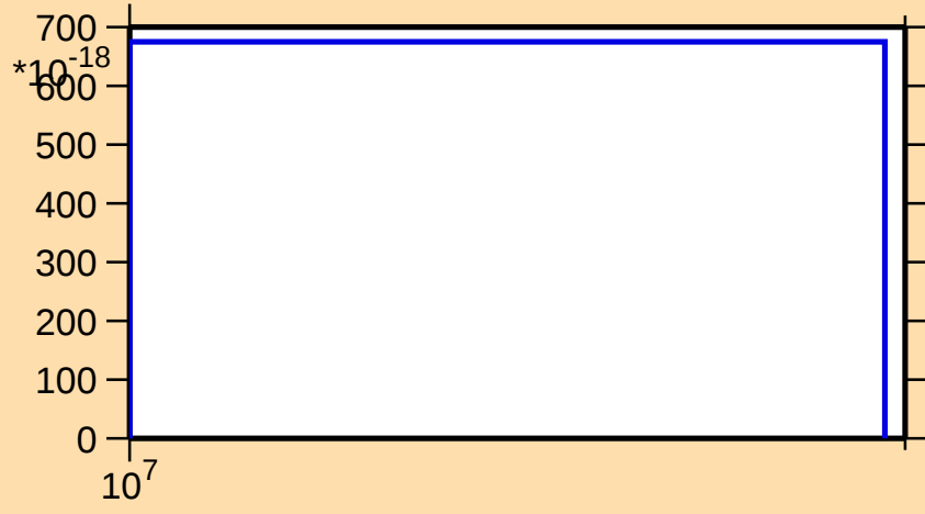
\sigma vs. E for ^{60}\text{Fe}(\text{n},\text{nd})
