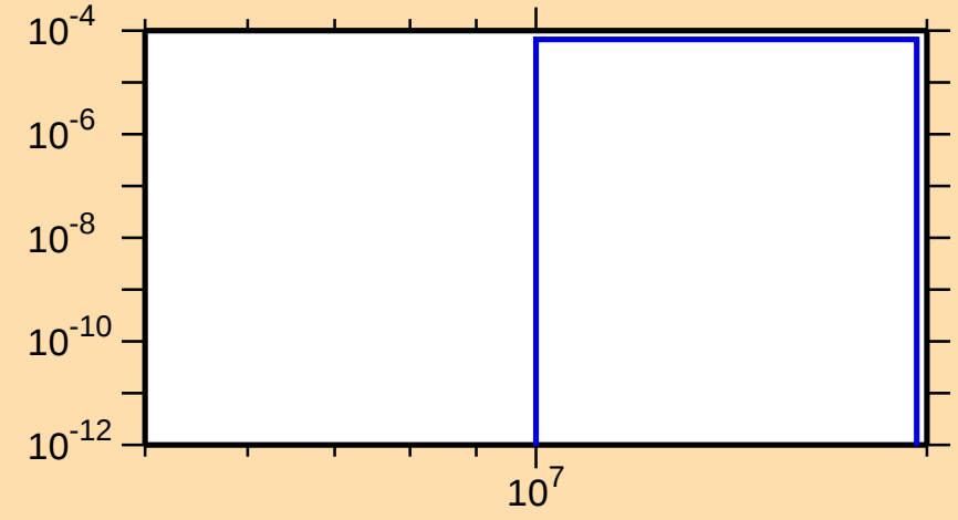
\sigma vs. E for ^{60}\text{Fe}(n,n\alpha)
