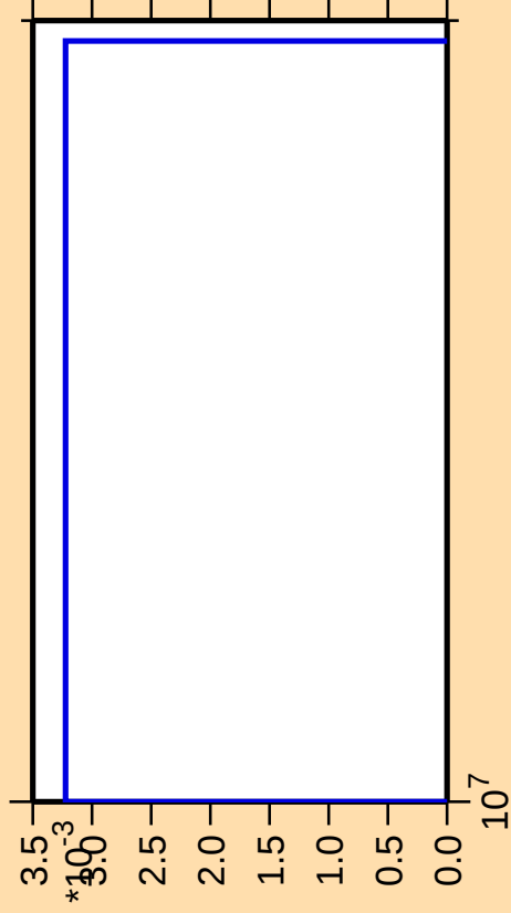
\Delta\sigma/\sigma vs. E for ^{60}\text{Fe}(\text{n},\text{nd})
