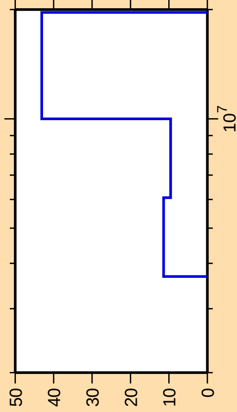
\Delta\sigma/\sigma vs. E for ^{60}\text{Fe}(\text{n},\text{ncont.})
