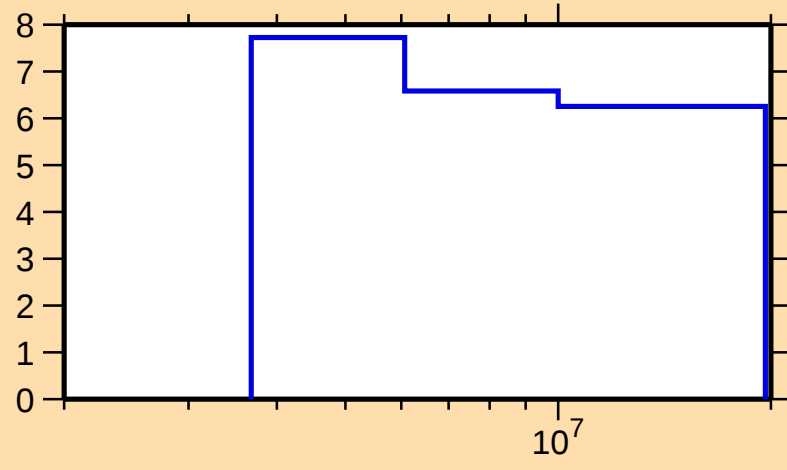
\Delta\sigma/\sigma vs. E for ^{60}\text{Fe}(\text{n},\text{nonel.})
