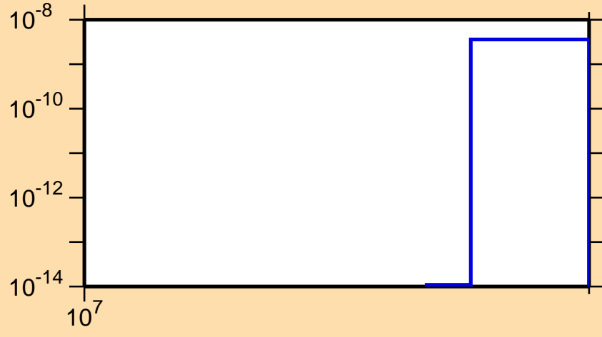
\sigma vs. E for ^{61}\text{Fe}(n,2n\alpha)
