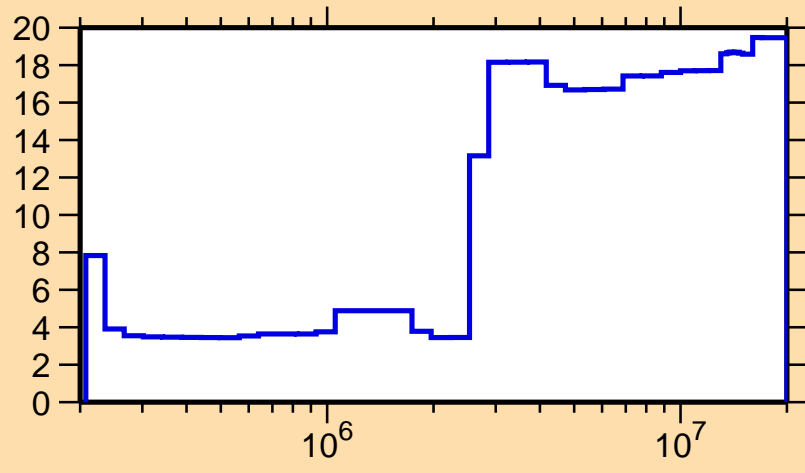
\Delta\sigma/\sigma vs. E for ^{61}\text{Fe}(n,n_1)
