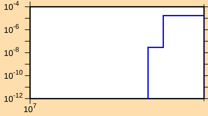
\sigma vs. E for ^{64}\text{Fe}(n,np)
