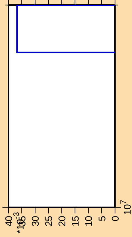
\Delta\sigma/\sigma vs. E for ^{64}\text{Fe}(n,\text{nd})
