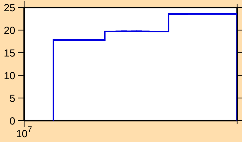
\Delta\sigma/\sigma vs. E for ^{64}\text{Fe}(n,2n)
