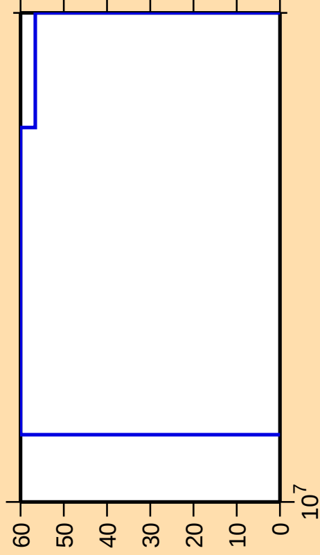
\Delta\sigma/\sigma vs. E for ^{64}\text{Fe}(\text{n,p})
