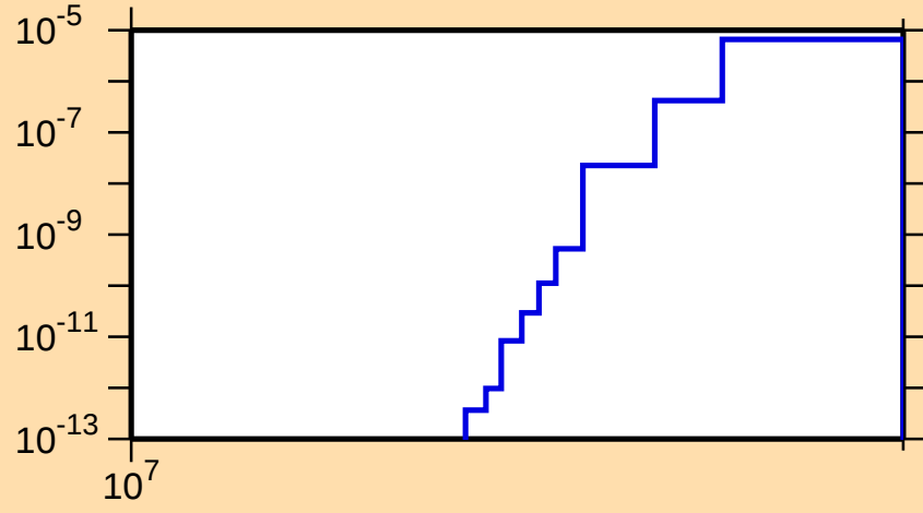
\sigma vs. E for ^{64}\text{Fe}(n,n\alpha)
