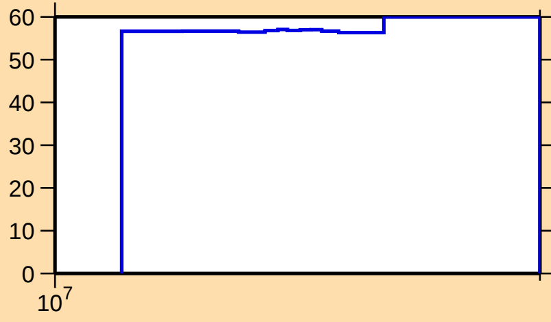
\Delta\sigma/\sigma vs. E for ^{64}\text{Fe}(\text{n,el.})
