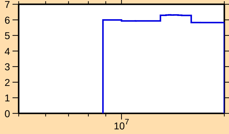
\Delta\sigma/\sigma vs. E for ^{65}\text{Fe}(n,\text{nonel.})
