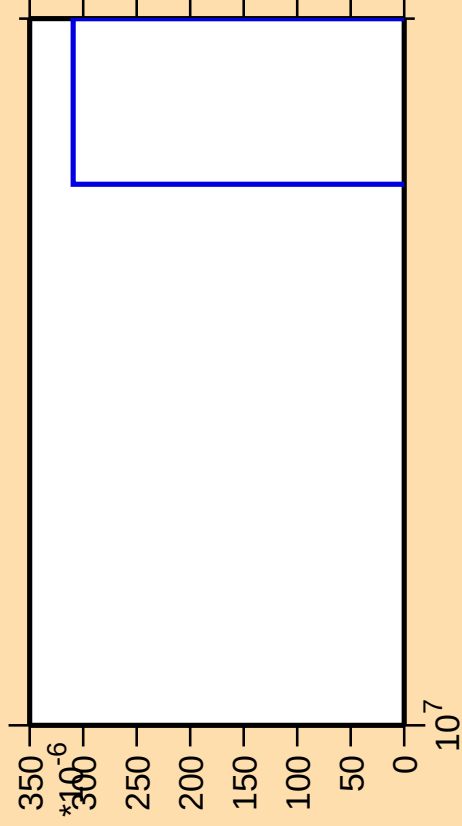
\Delta\sigma/\sigma vs. E for ^{65}\text{Fe}(n,2np)
