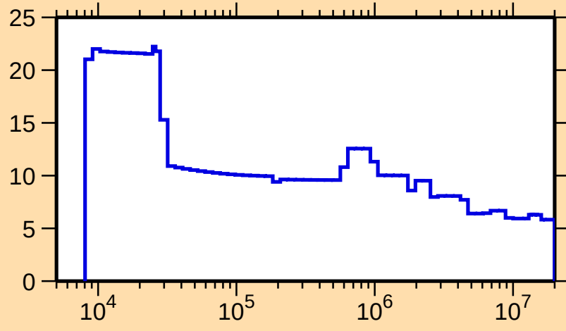
\Delta\sigma/\sigma vs. E for ^{65}\text{Fe}(n,\text{nonel.})
