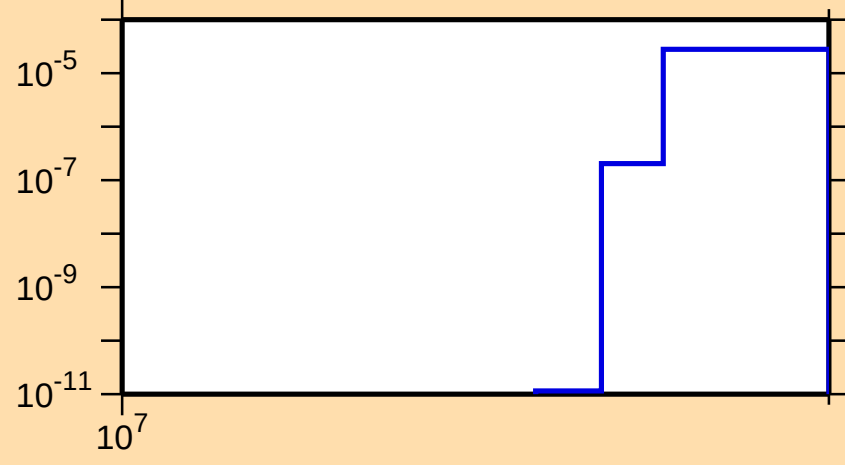
\sigma vs. E for ^{65}\text{Fe}(n,np)
