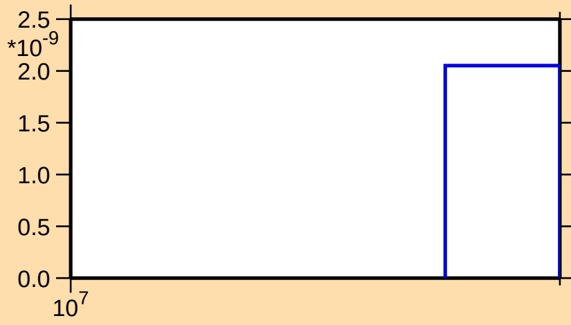
\sigma vs. E for ^{65}\text{Fe}(n,\text{nt})
