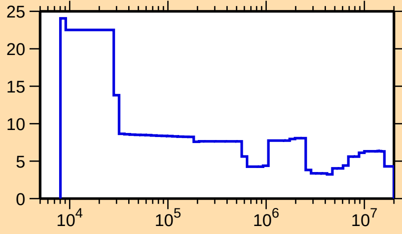
\Delta\sigma/\sigma vs. E for ^{65}\text{Fe}(n,\text{tot.})
