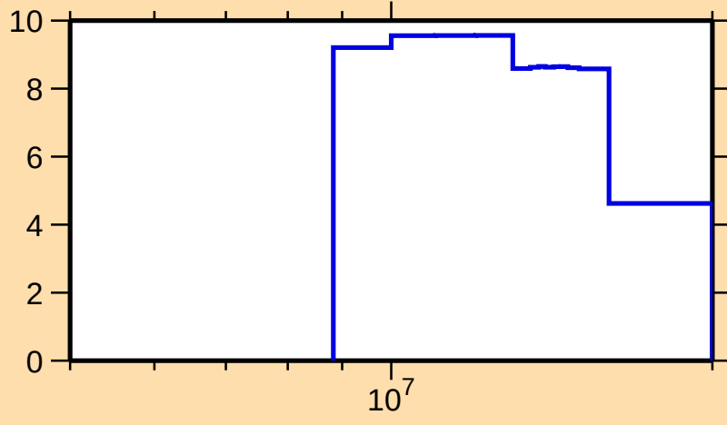
\Delta\sigma/\sigma vs. E for ^{65}\text{Fe}(n,\text{el.})
