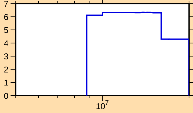
\Delta\sigma/\sigma vs. E for ^{65}\text{Fe}(n,\text{tot.})
