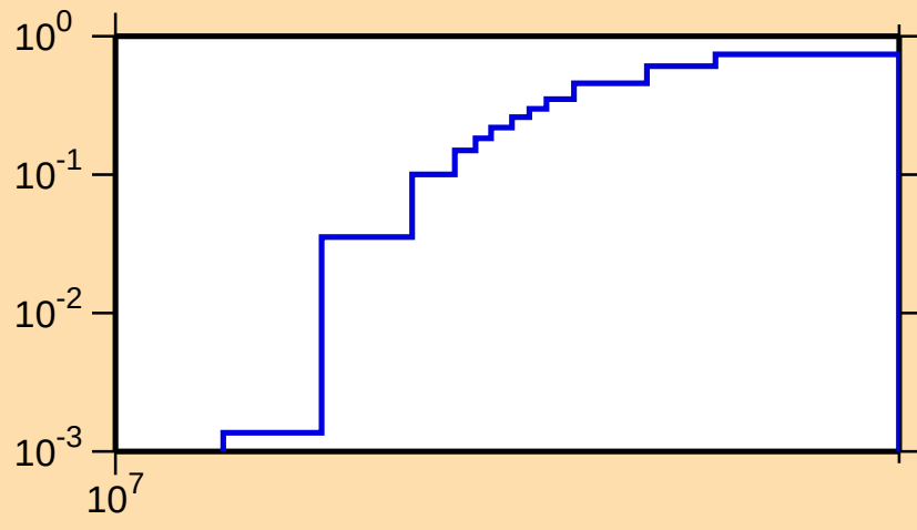
\sigma vs. E for ^{65}\text{Fe}(n,3n)
