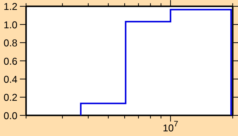
\sigma vs. E for ^{65}\text{Fe}(n,2n)
