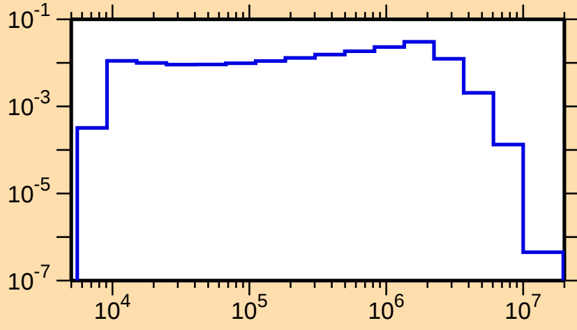
\sigma vs. E for ^{65}\text{Fe}(n,n_1)
