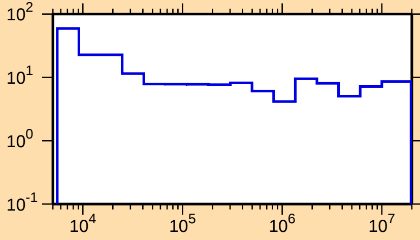
\Delta\sigma/\sigma vs. E for ^{65}\text{Fe}(\text{n,el.})
