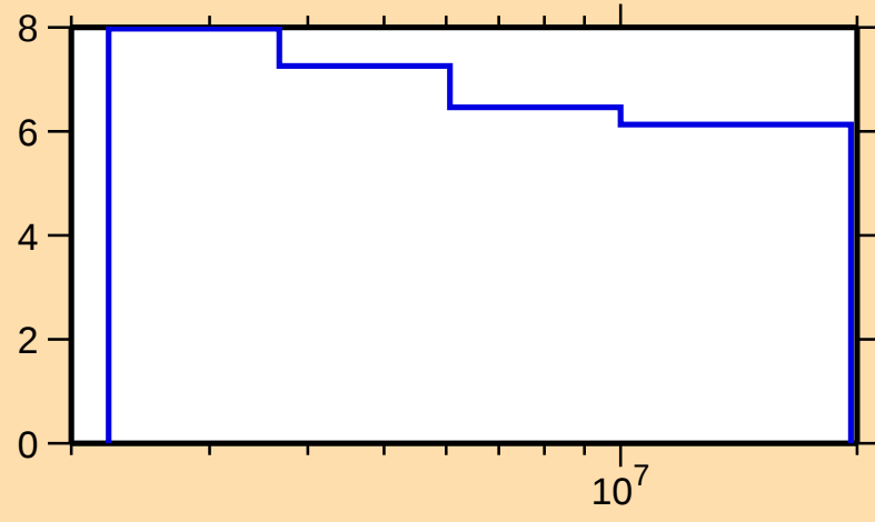
\Delta\sigma/\sigma vs. E for ^{65}\text{Fe}(\text{n},\text{nonel.})
