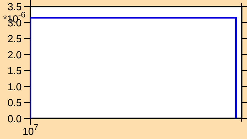
\sigma vs. E for ^{65}\text{Fe}(n,t)
