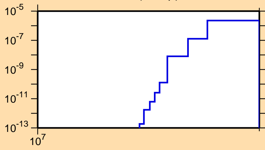
\sigma vs. E for ^{246}\text{Fm}(n,2np)
