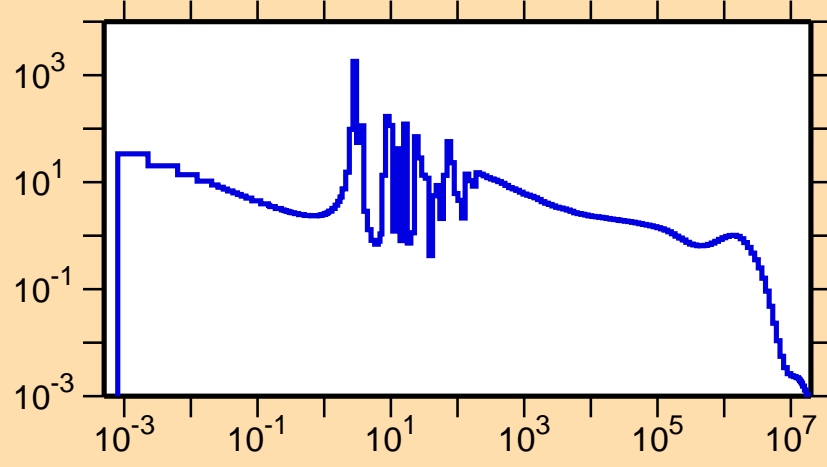
\sigma vs. E for ^{246}\text{Fm}(n,\gamma)
