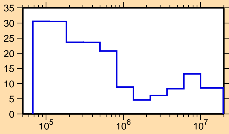
\Delta\sigma/\sigma vs. E for ^{246}\text{Fm}(n,\text{tot.})
