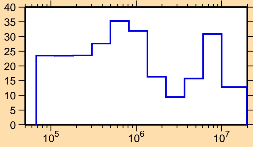
\Delta\sigma/\sigma vs. E for ^{246}\text{Fm}(n, el.)
