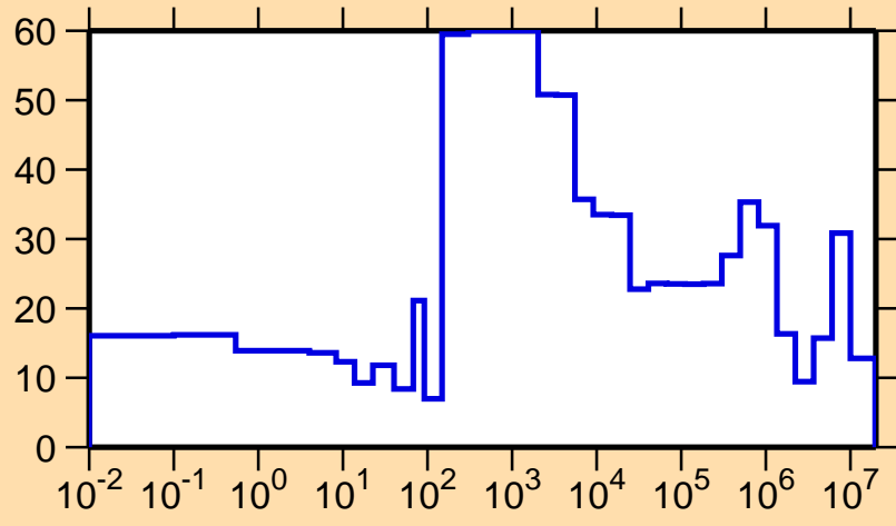
\Delta\sigma/\sigma vs. E for ^{246}\text{Fm}(n,\text{el.})
