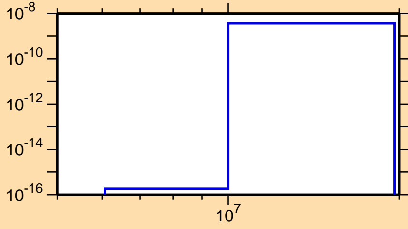
\sigma vs. E for ^{246}\text{Fm}(\text{mt117})
