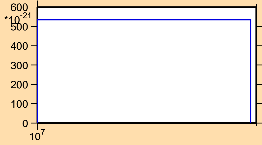
\sigma vs. E for ^{246}\text{Fm} (mt 42)
