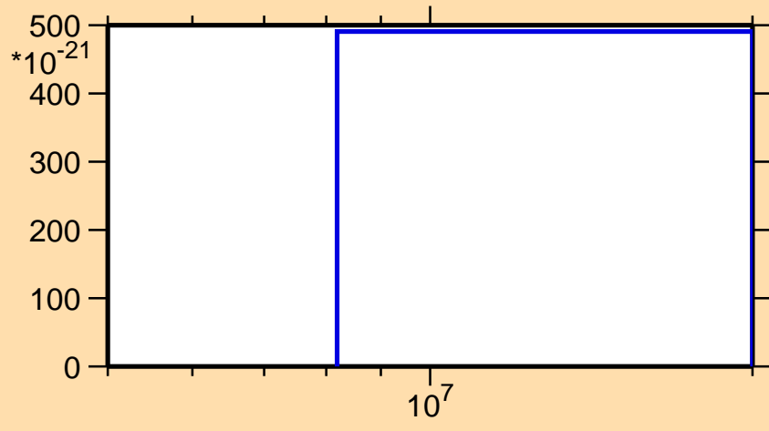
\sigma vs. E for ^{246}\text{Fm} (mt 42)
