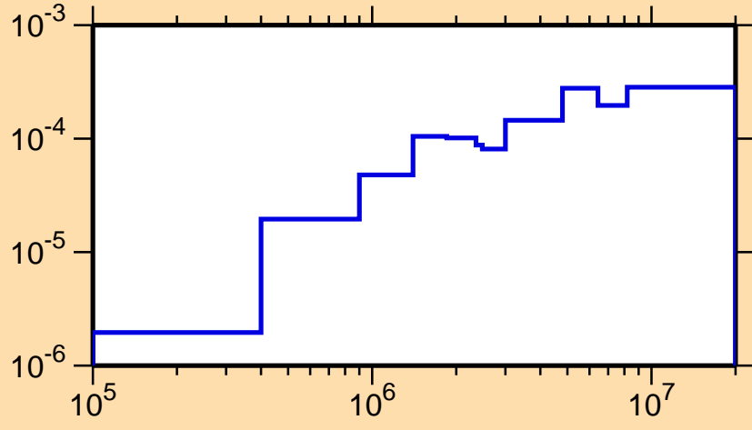
\sigma vs. E for ^{246}\text{Fm}(n,n\alpha)
