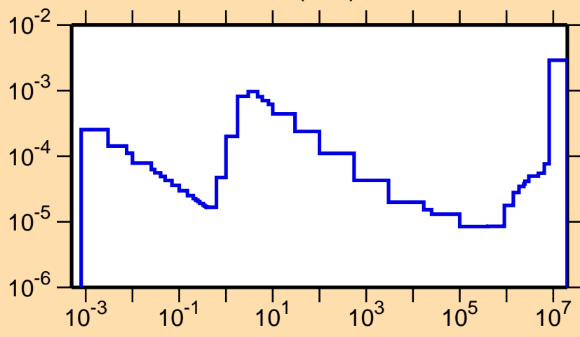
\sigma vs. E for ^{246}\text{Fm}(n,\alpha)
