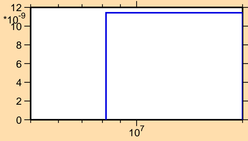
\sigma vs. E for ^{246}\text{Fm}(n,nd)
