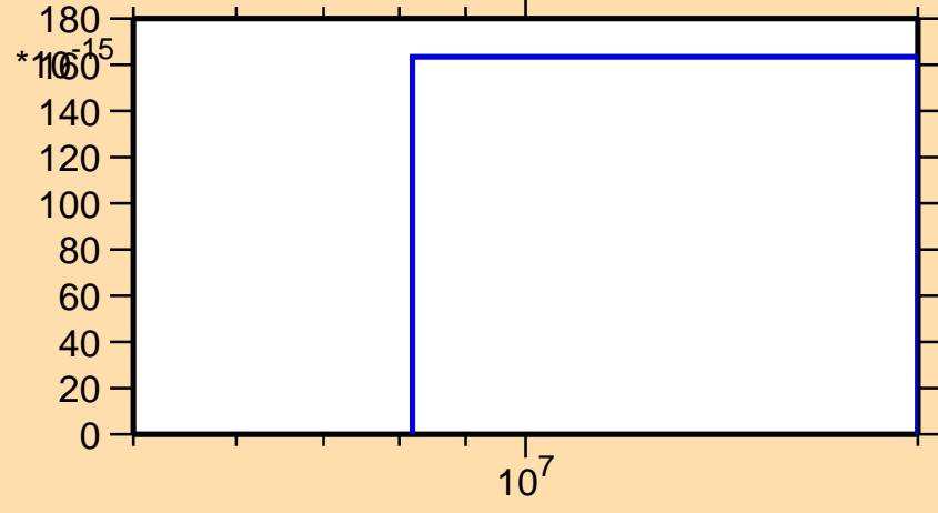
\sigma vs. E for ^{246}\text{Fm}(n,pd)
