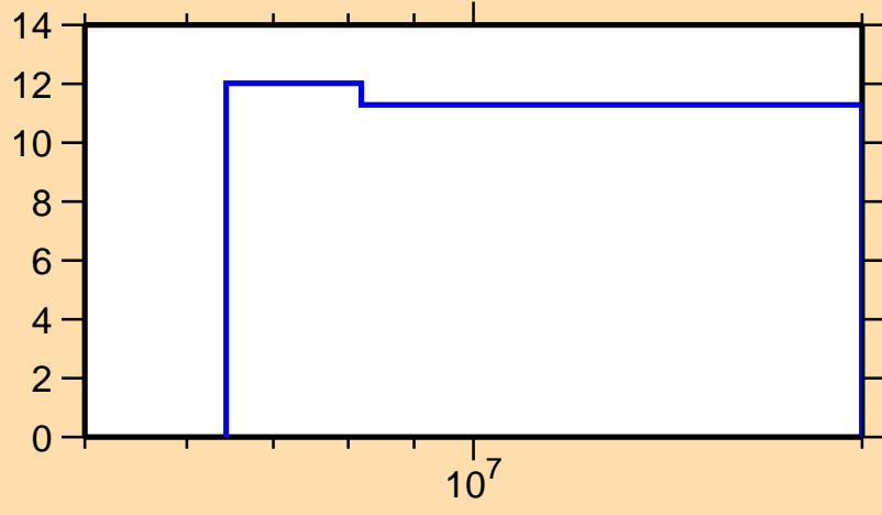
\Delta\sigma/\sigma vs. E for ^{246}\text{Fm}(n,\text{nonel.})
