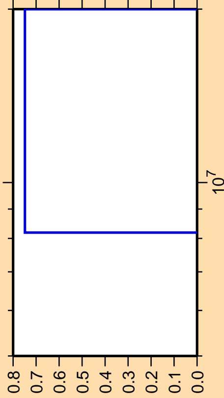
\Delta\sigma/\sigma vs. E for ^{246}\text{Fm}(n,pd)
