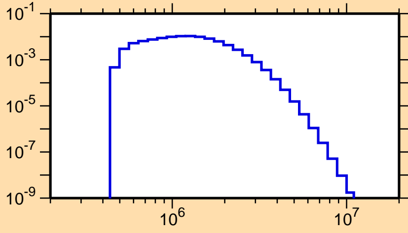
\sigma vs. E for ^{247}\text{Fm}(n,n_2)
