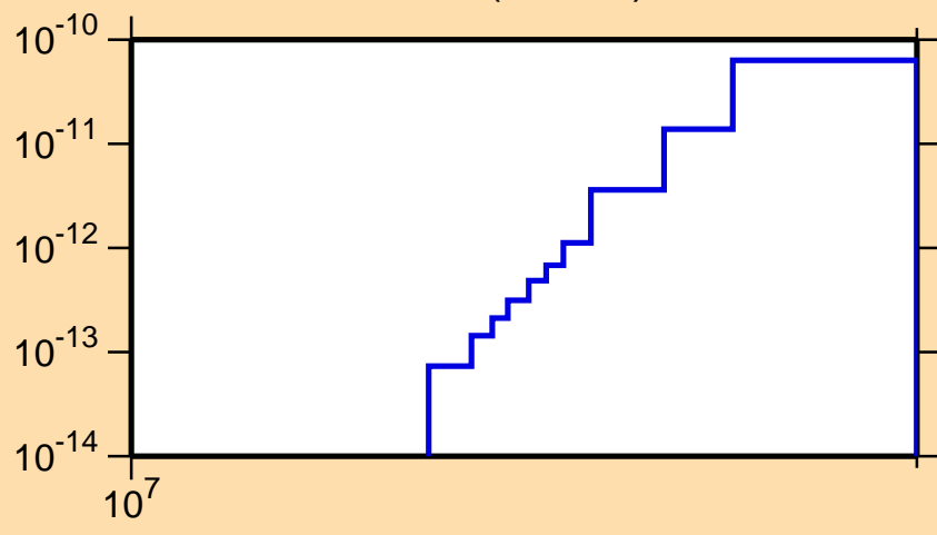
\sigma vs. E for ^{247}\text{Fm}(\text{mt117})
