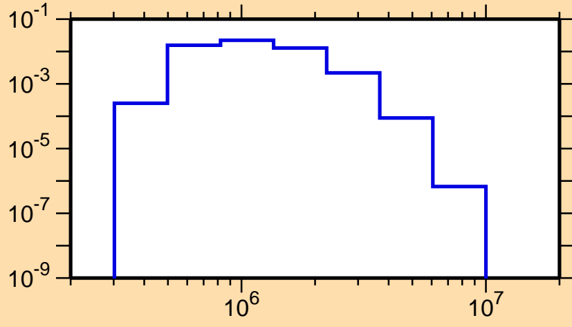
\sigma vs. E for ^{247}\text{Fm}(n,n_3)
