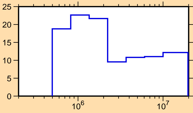
\Delta\sigma/\sigma vs. E for ^{247}\text{Fm}(n,nonel.)
