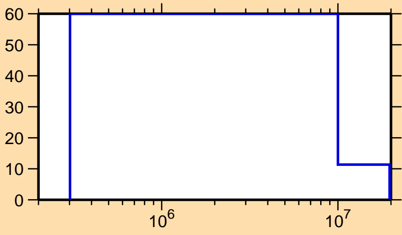
\Delta\sigma/\sigma vs. E for ^{247}\text{Fm}(n,n_1)
