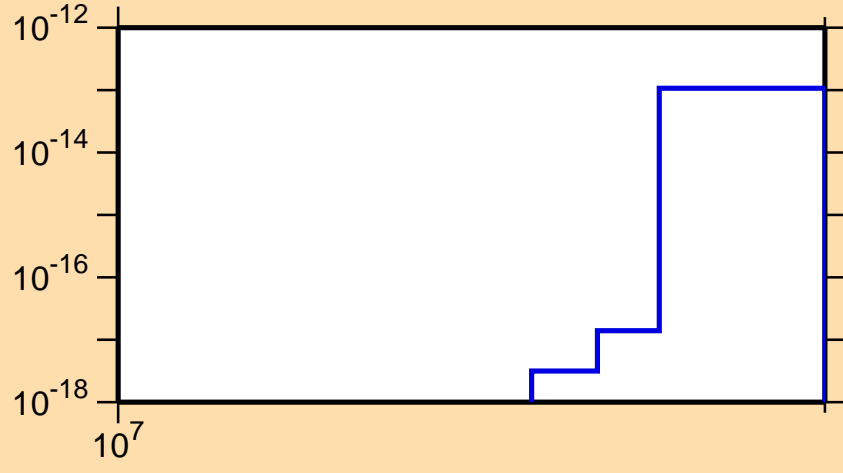
\sigma vs. E for ^{247}\text{Fm} (mt 11)
