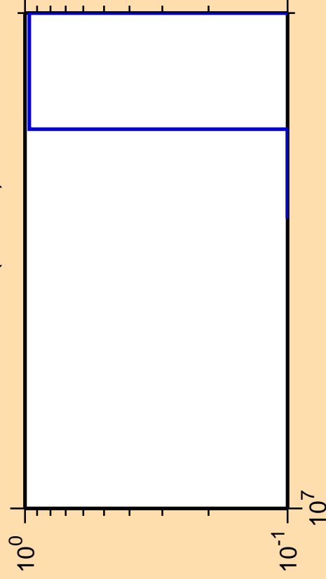
\Delta\sigma/\sigma vs. E for ^{247}\text{Fm} (mt 11)
