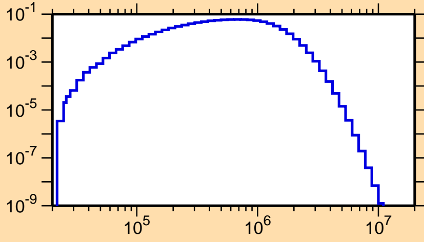
\sigma vs. E for ^{247}\text{Fm}(n,n_4)
