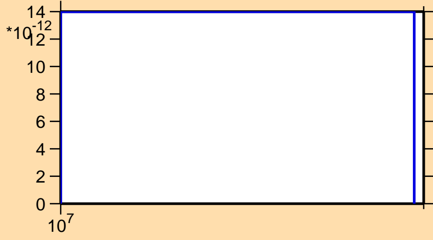
\sigma vs. E for ^{247}\text{Fm}(\text{mt117})
