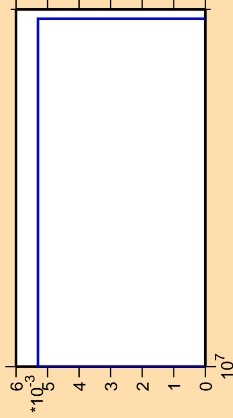
\Delta\sigma/\sigma vs. E for ^{247}\text{Fm} (mt 11)
