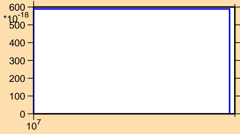
\sigma vs. E for ^{247}\text{Fm} (mt 11)
