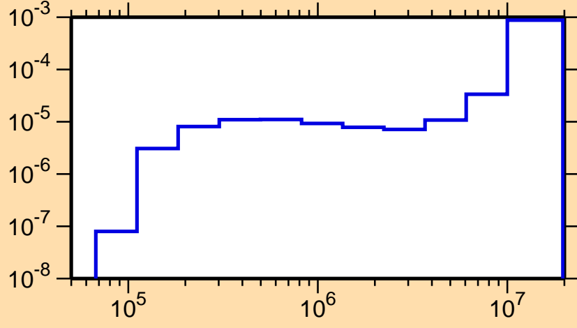
\sigma vs. E for ^{247}\text{Fm}(n,n\alpha)
