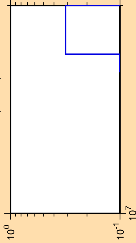
\Delta\sigma/\sigma vs. E for ^{250}\text{Fm} (mt 11)
