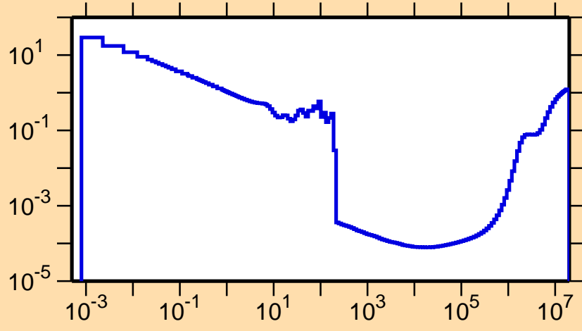
\sigma vs. E for ^{250}\text{Fm}(n,f)
