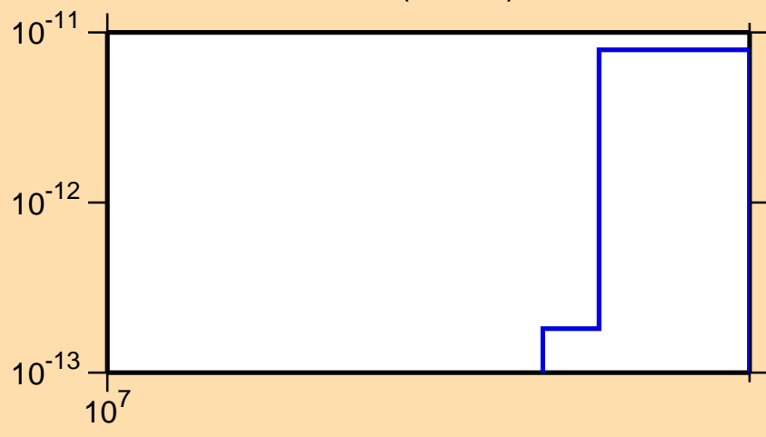
\sigma vs. E for ^{250}\text{Fm} (mt 34)
