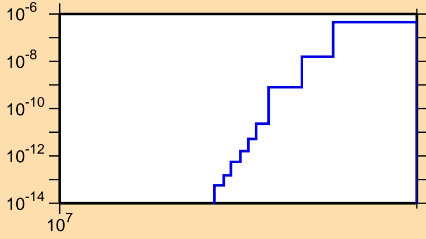
\sigma vs. E for ^{252}\text{Fm}(n,\text{nd})
