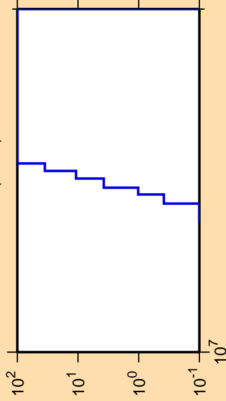
\Delta\sigma/\sigma vs. E for ^{252}\text{Fm}(n,\text{nd})
