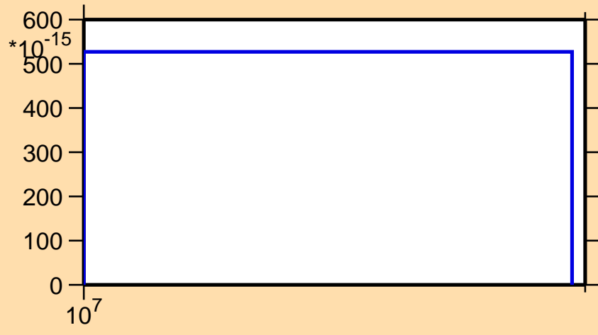
\sigma vs. E for ^{252}\text{Fm}(n,p\alpha)
