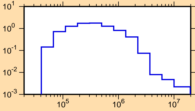
\sigma vs. E for ^{252}\text{Fm}(n,n_1)
