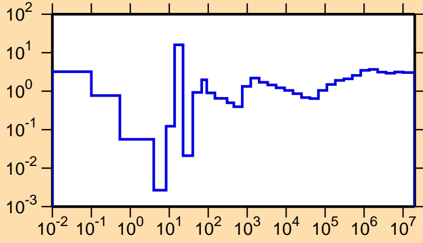
\sigma vs. E for ^{252}\text{Fm}(n,\text{nonel.})
