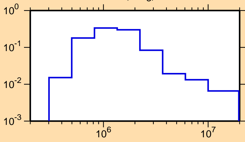
\sigma vs. E for ^{252}\text{Fm}(n,n_3)
