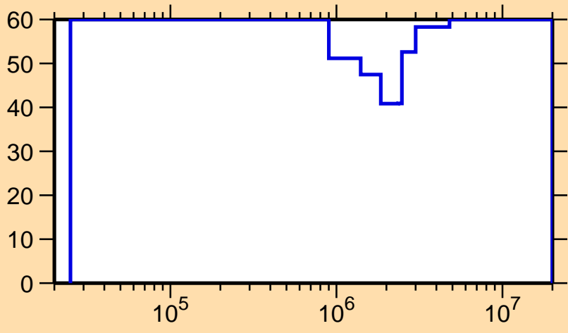
\Delta\sigma/\sigma vs. E for ^{252}\text{Fm}(n,\text{inel.})
