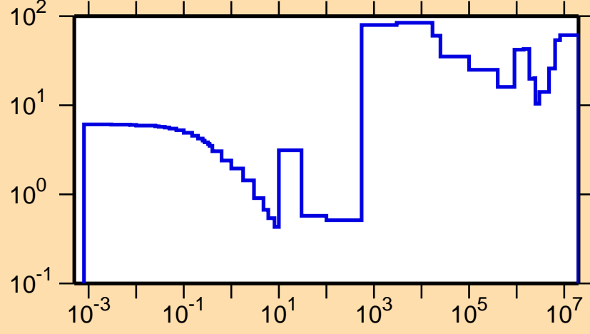
\Delta\sigma/\sigma vs. E for ^{252}\text{Fm}(n,el.)
