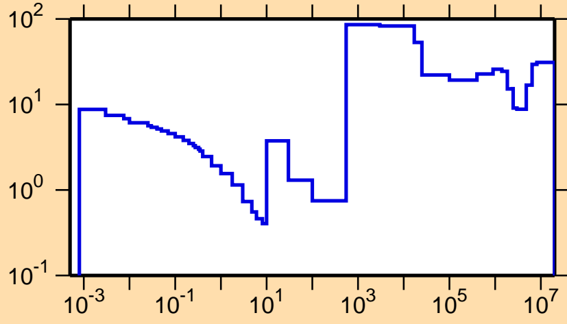
\Delta\sigma/\sigma vs. E for ^{252}\text{Fm}(n,tot.)
