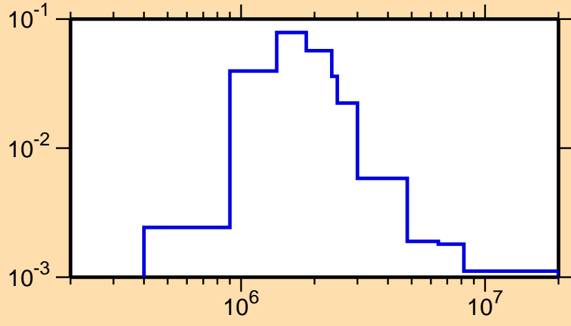
\sigma vs. E for ^{252}\text{Fm}(n,n_4)
