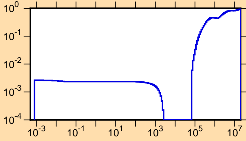
\mu vs. E for ^{253}\text{Fm}(\text{mt251})
