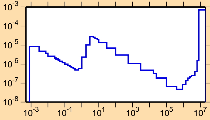
\sigma vs. E for ^{253}\text{Fm}(n,\alpha)
