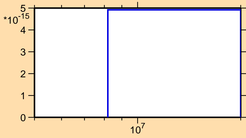
\sigma vs. E for ^{253}\text{Fm} (mt 34)
