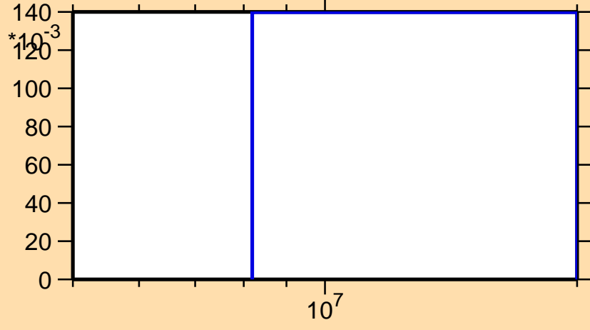
\sigma vs. E for ^{253}\text{Fm}(n,3n)
