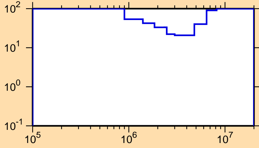
\Delta\sigma/\sigma vs. E for ^{253}\text{Fm}(n,ncont.)
