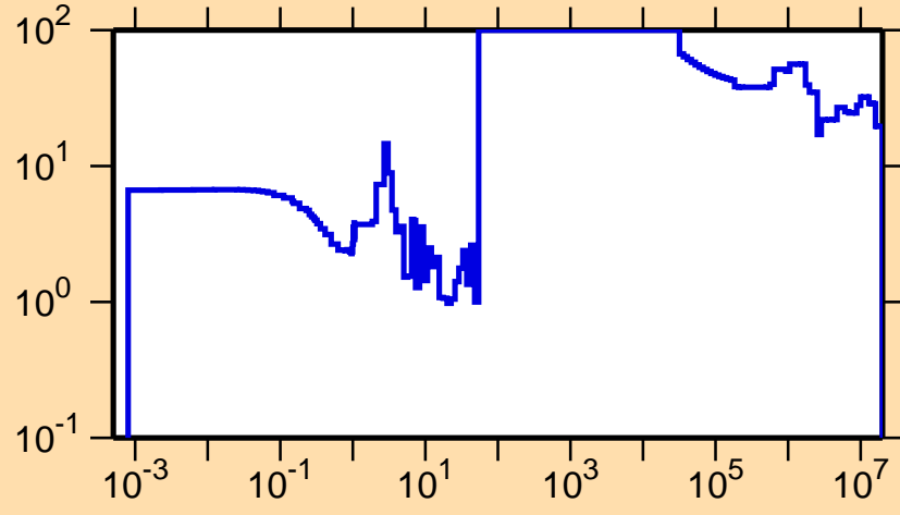
\Delta\sigma/\sigma vs. E for ^{255}\text{Fm}(n,el.)
