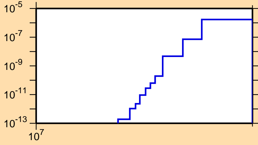
\sigma vs. E for ^{255}\text{Fm}(n,nt)
