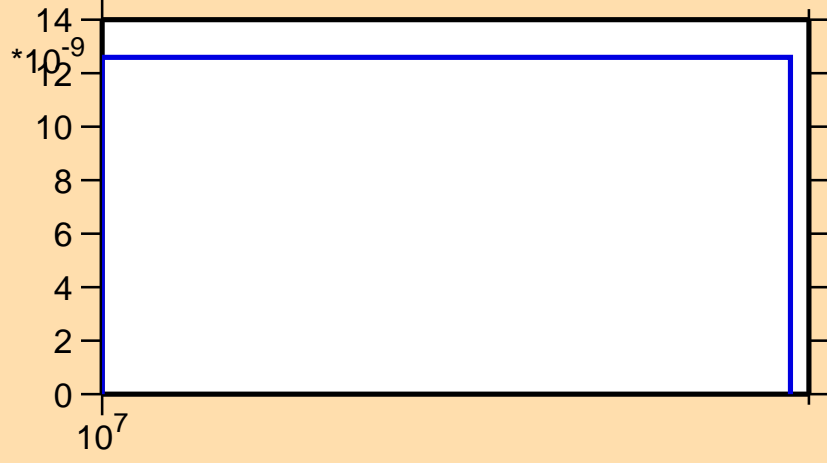
\sigma vs. E for ^{255}\text{Fm}(n,2np)
