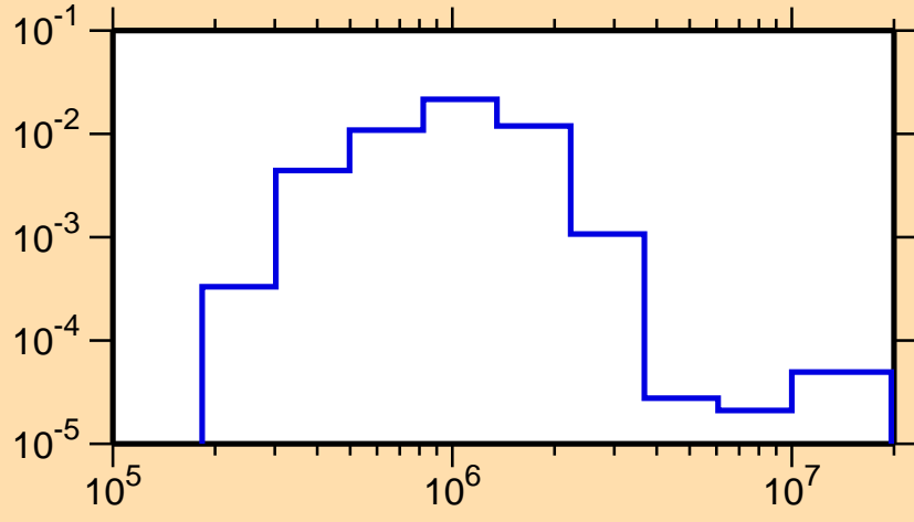
\sigma vs. E for ^{255}\text{Fm}(n,n_3)
