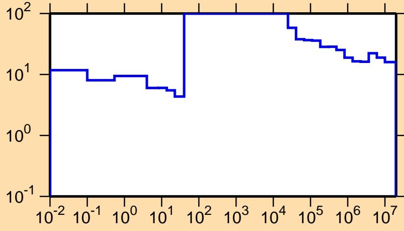
\Delta\sigma/\sigma vs. E for ^{255}\text{Fm}(n,tot.)
