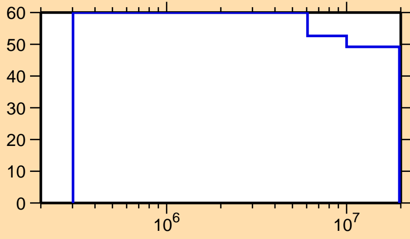
\Delta\sigma/\sigma vs. E for ^{255}\text{Fm}(n, \text{inel.})
