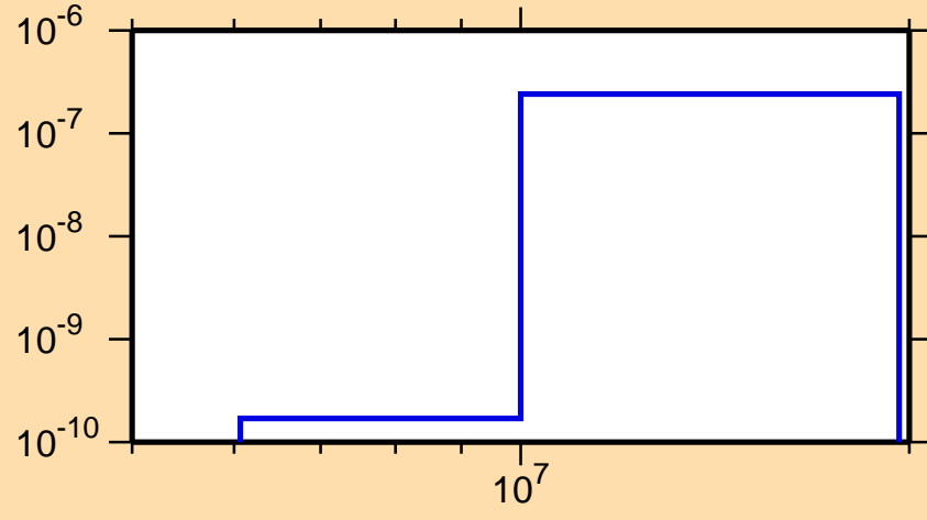
\sigma vs. E for ^{255}\text{Fm}(n,2n\alpha)
