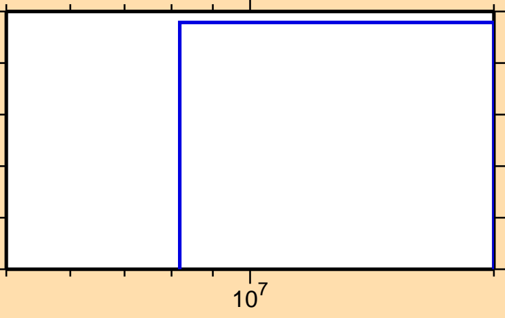
\sigma vs. E for ^{255}\text{Fm}(n,\text{nd})
