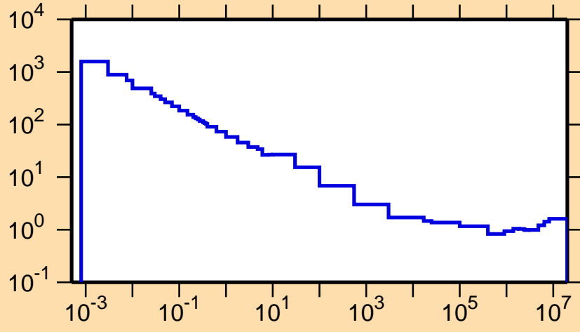
\sigma vs. E for ^{255}\text{Fm}(n,f)
