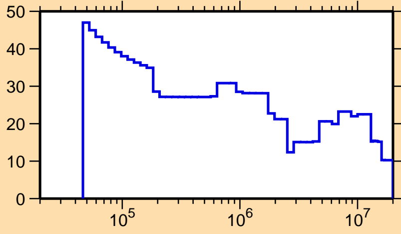
\Delta\sigma/\sigma vs. E for ^{256}\text{Fm}(n,\text{tot.})
