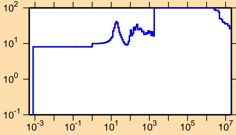
\Delta\sigma/\sigma vs. E for ^{256}\text{Fm}(n,f)
