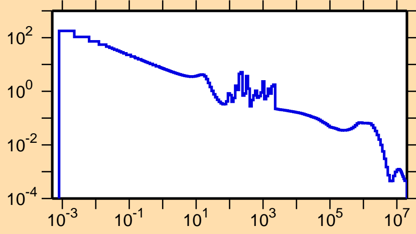
\sigma vs. E for ^{256}\text{Fm}(n,\gamma)
