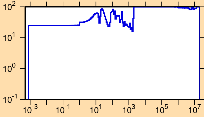
\Delta\sigma/\sigma vs. E for ^{256}\text{Fm}(n,\gamma)
