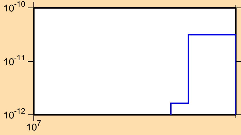
\sigma vs. E for ^{256}\text{Fm}(n,\text{He3})
