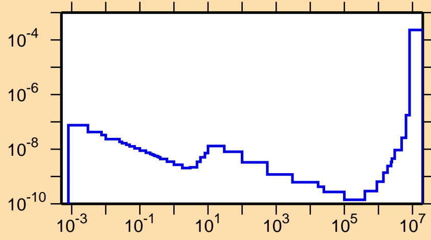
\sigma vs. E for ^{256}\text{Fm}(n,\alpha)
