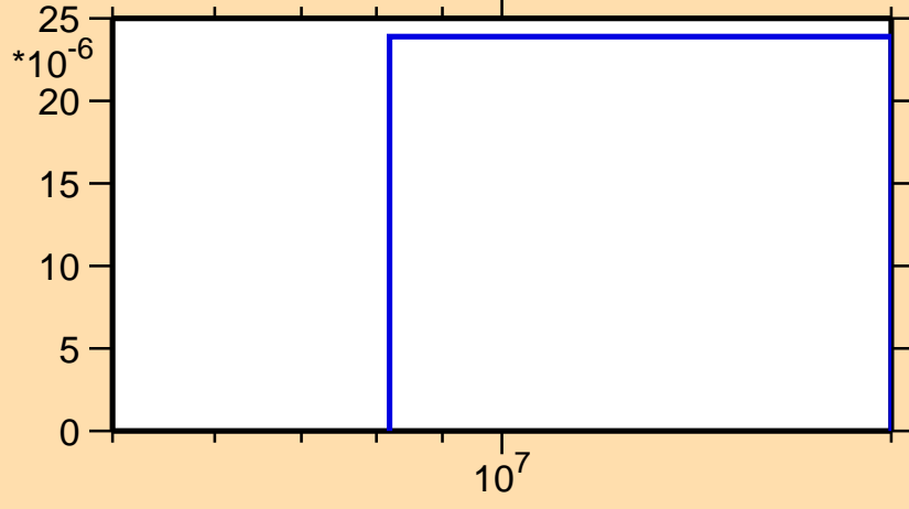
\sigma vs. E for ^{256}\text{Fm}(n,np)
