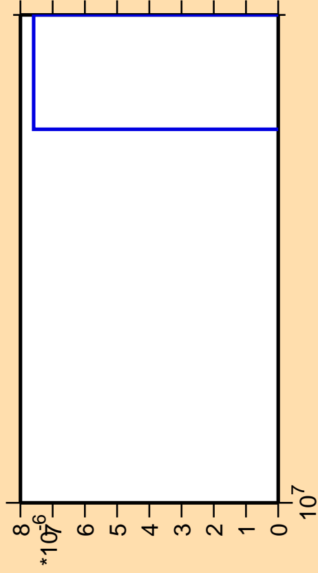
\Delta\sigma/\sigma vs. E for ^{257}\text{Fm} (mt 11)
