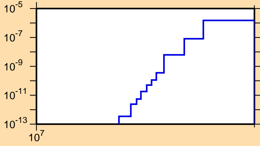
\sigma vs. E for ^{257}\text{Fm}(n,\text{nd})
