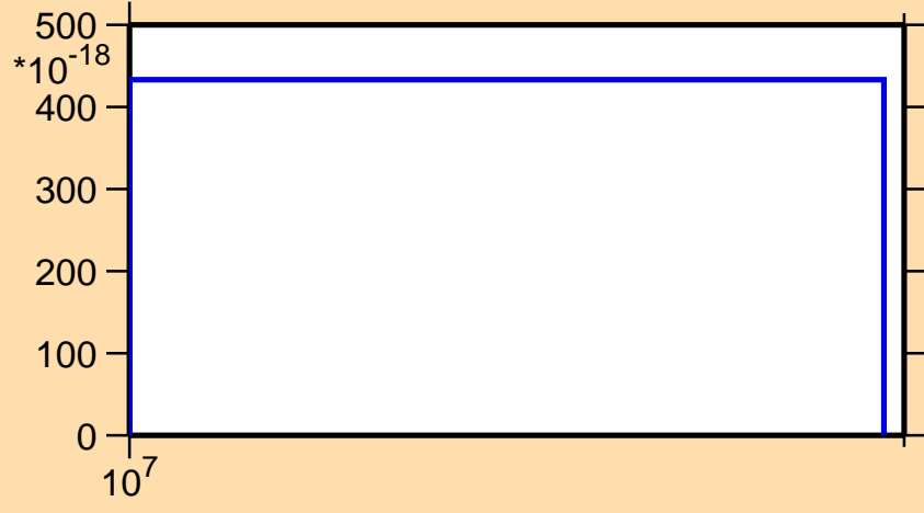
\sigma vs. E for ^{257}\text{Fm} (mt 11)
