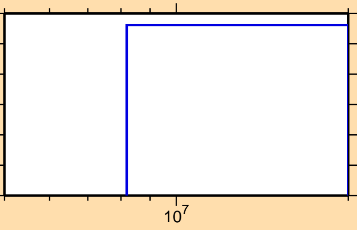
\sigma vs. E for ^{257}\text{Fm}(n,np)
