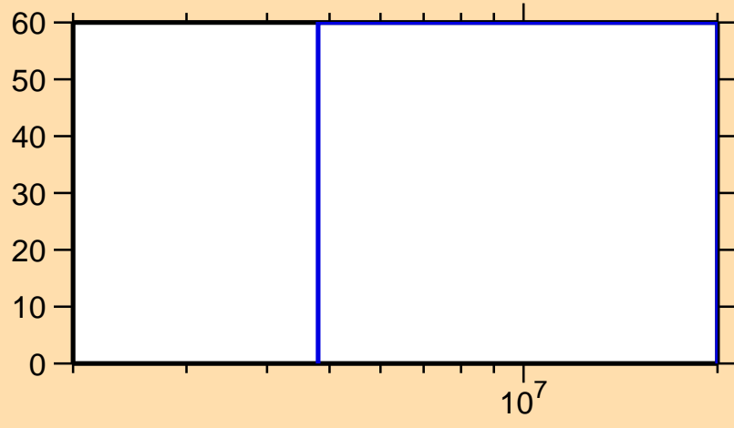
\Delta\sigma/\sigma vs. E for ^{257}\text{Fm}(n,2n)
