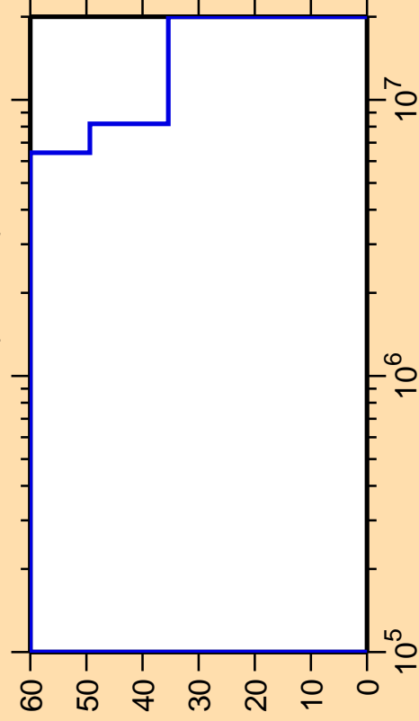
\Delta\sigma/\sigma vs. E for ^{257}\text{Fm}(n,\text{inel.})
