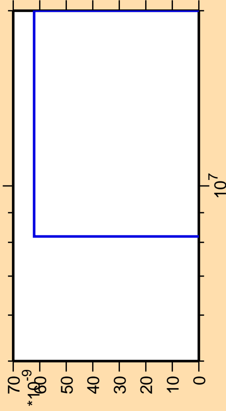
\Delta\sigma/\sigma vs. E for ^{257}\text{Fm}(\text{mt } 11)
