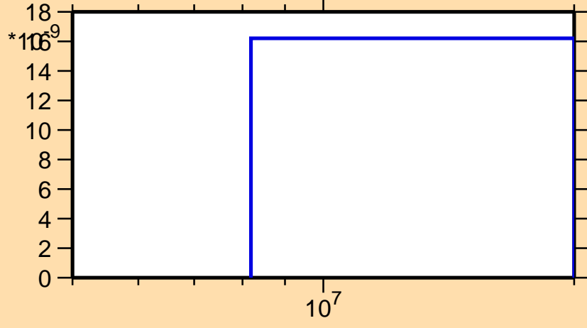
\sigma vs. E for ^{257}\text{Fm}(n,nd)
