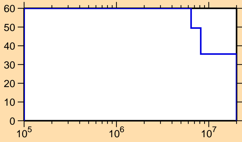
\Delta\sigma/\sigma vs. E for ^{257}\text{Fm}(n,ncont.)
