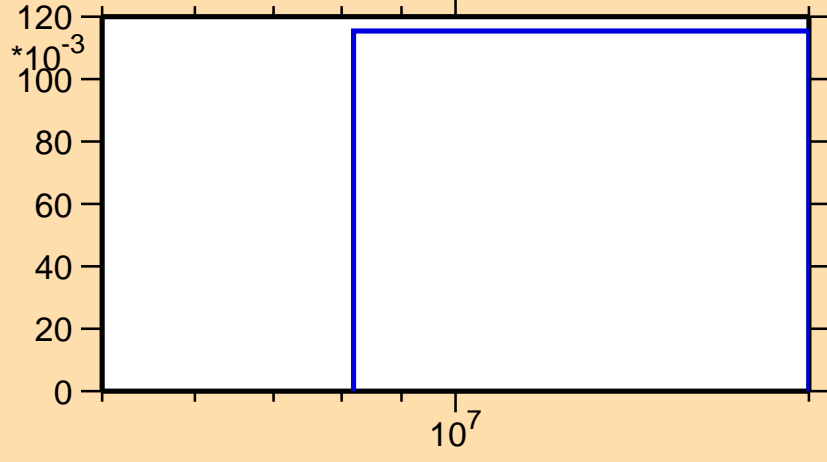
\sigma vs. E for ^{257}\text{Fm}(n,3n)
