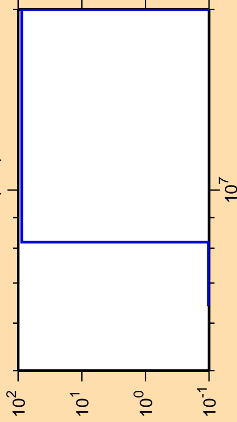
\Delta\sigma/\sigma vs. E for ^{257}\text{Fm}(n,d)
