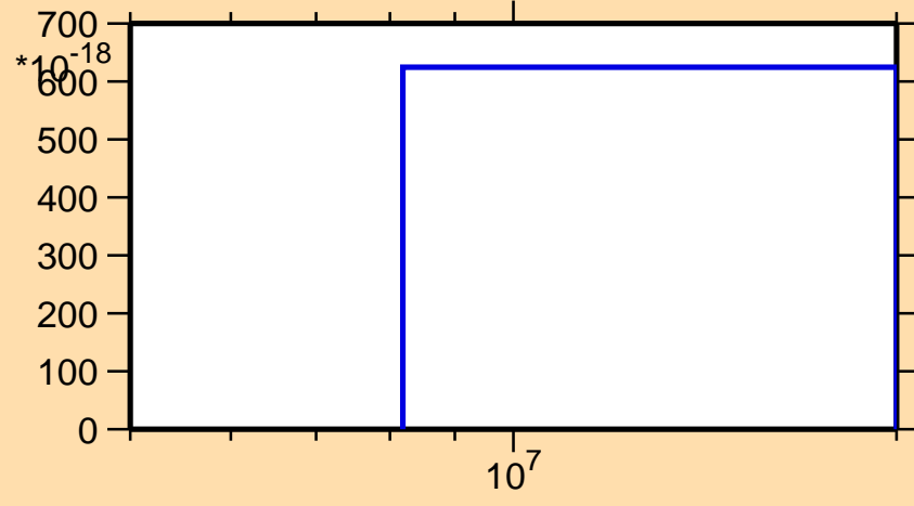
\sigma vs. E for ^{257}\text{Fm}(\text{mt } 11)
