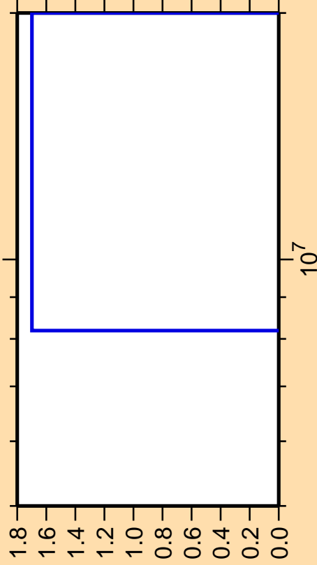
\Delta\sigma/\sigma vs. E for ^{257}\text{Fm}(n,\text{He}3)
