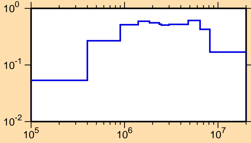
\sigma vs. E for ^{257}\text{Fm}(n,\text{inel.})
