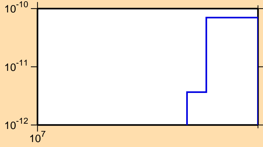
\sigma vs. E for ^{259}\text{Fm}(n,3n\alpha)
