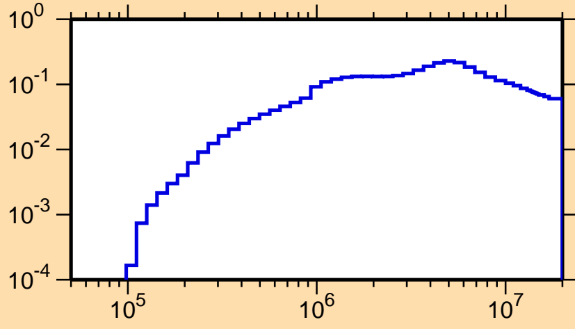
\sigma vs. E for ^{259}\text{Fm}(n,n\text{cont.})
