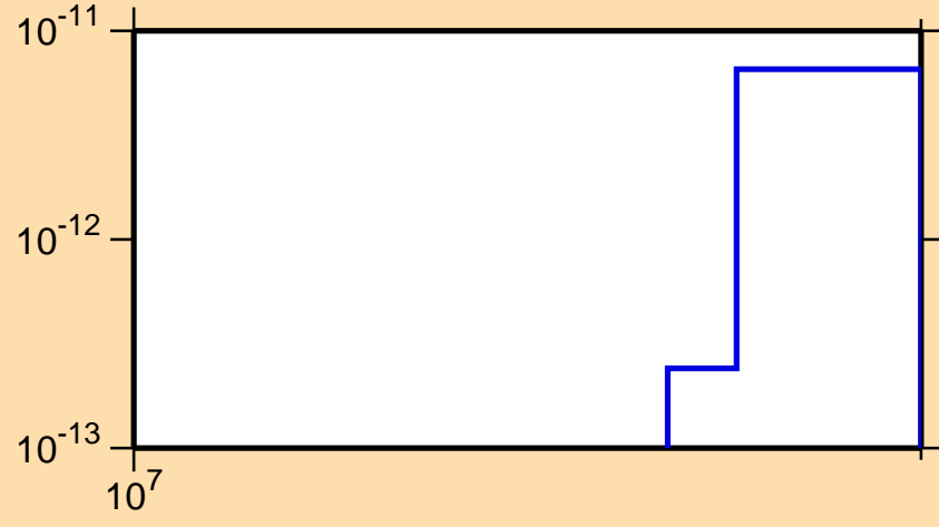
\sigma vs. E for ^{259}\text{Fm}(n,\text{He3})
