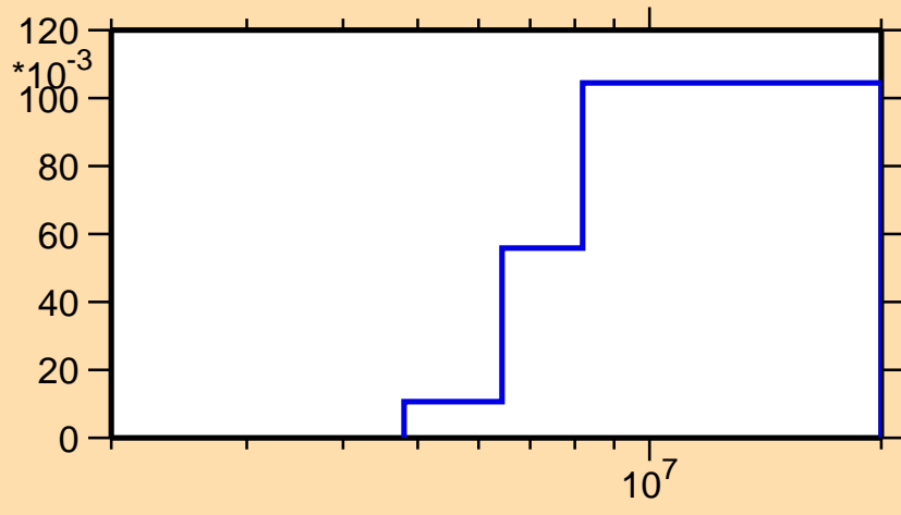
\sigma vs. E for ^{259}\text{Fm}(n,2n)
