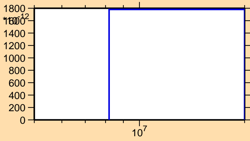
\sigma vs. E for ^{259}\text{Fm}(n,\text{nd})
