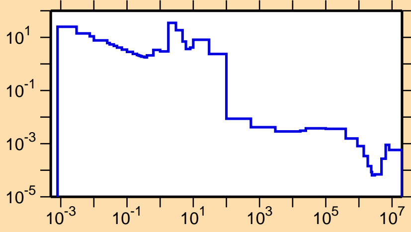
\sigma vs. E for ^{259}\text{Fm}(n,\gamma)
