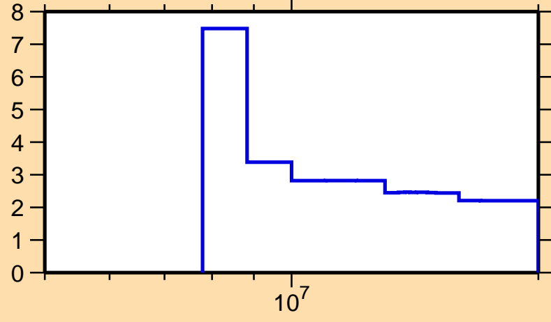
\Delta\sigma/\sigma vs. E for ^{204}\text{Fr}(n,\text{tot.})
