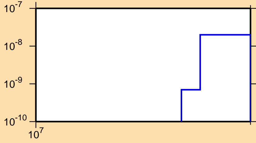
\sigma vs. E for ^{204}\text{Fr}(n,3n\alpha)
