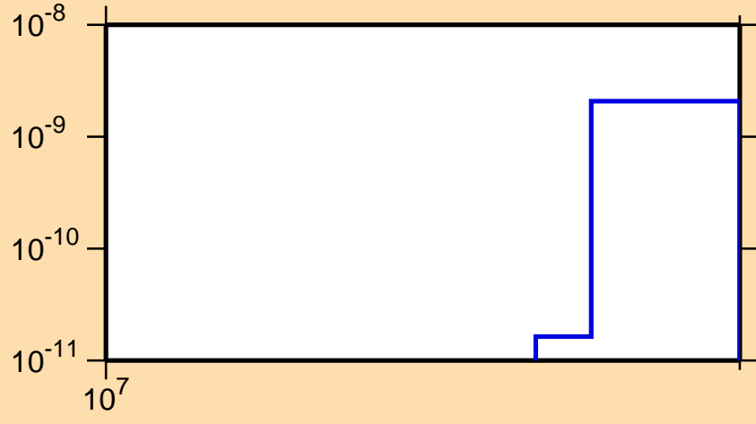
\sigma vs. E for ^{204}\text{Fr}(n,nt)
