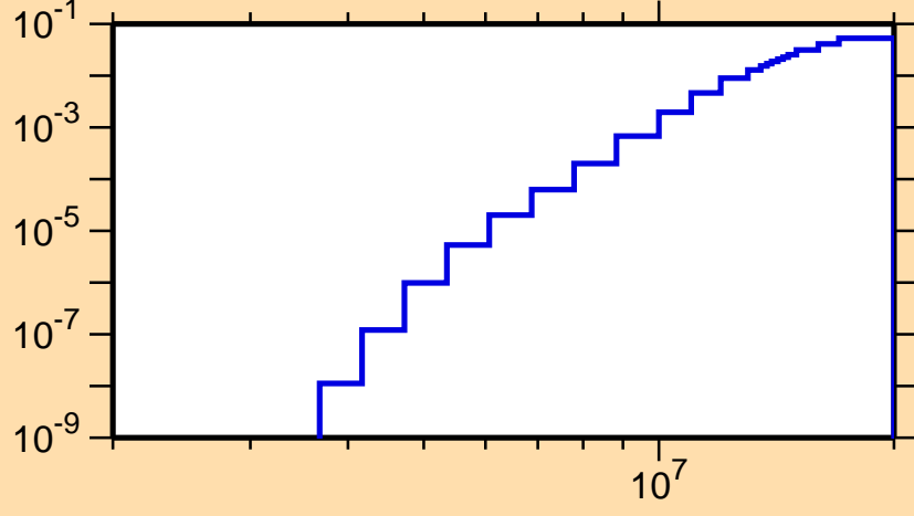
\sigma vs. E for ^{204}\text{Fr}(n,np)
