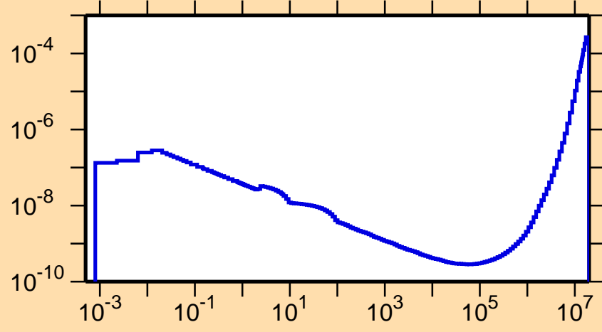
\sigma vs. E for ^{204}\text{Fr}(n,p\alpha)
