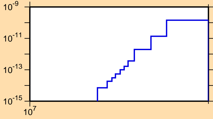
\sigma vs. E for ^{204}\text{Fr}(\text{mt } 34)
