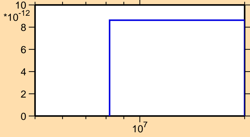
\sigma vs. E for ^{204}\text{Fr}(n,nt)
