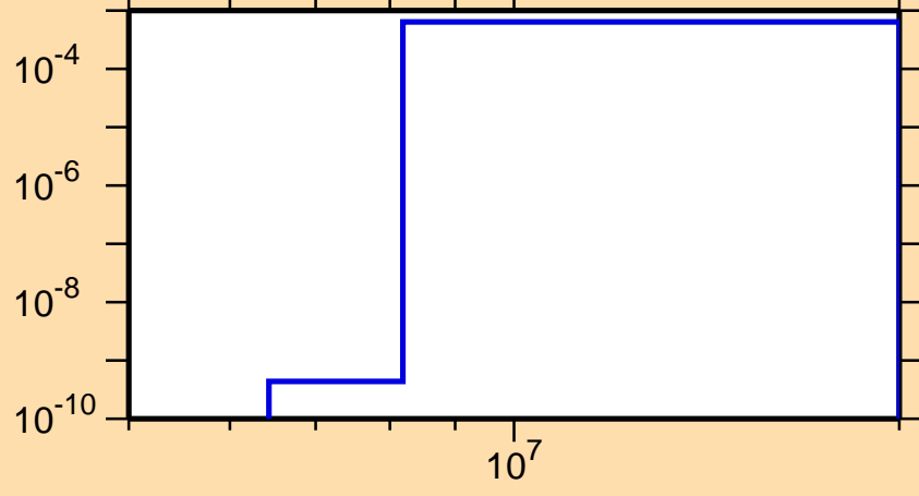
\sigma vs. E for ^{204}\text{Fr}(n,t)
