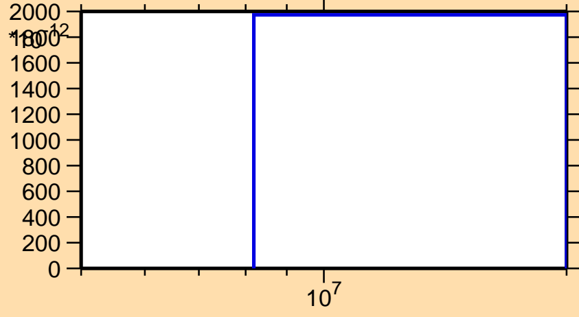
\sigma vs. E for ^{204}\text{Fr}(n,\text{pd})
