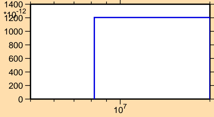
\sigma vs. E for ^{204}\text{Fr}(n,3n)
