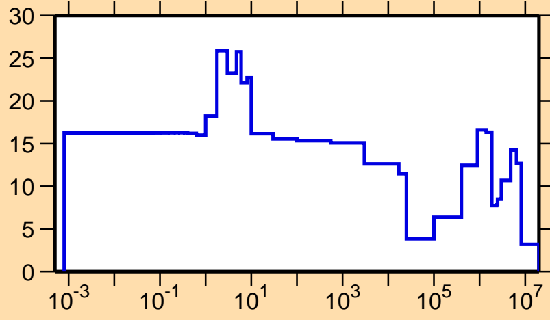
\Delta\sigma/\sigma vs. E for ^{204}\text{Fr}(n,\text{el.})
