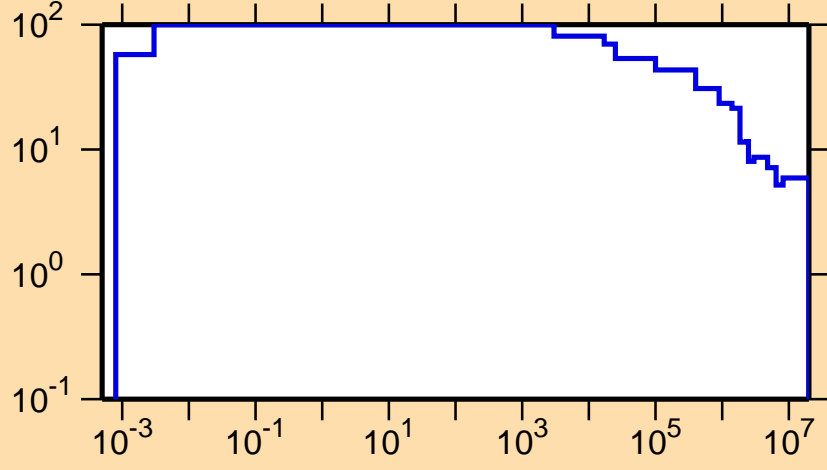
\Delta\sigma/\sigma vs. E for ^{204}\text{Fr}(n,\text{nonel.})
