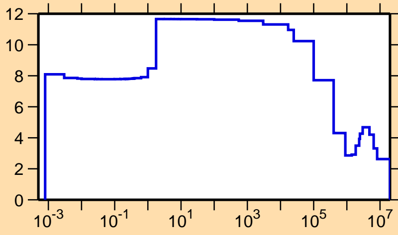
\sigma vs. E for ^{204}\text{Fr}(n,\text{el.})
