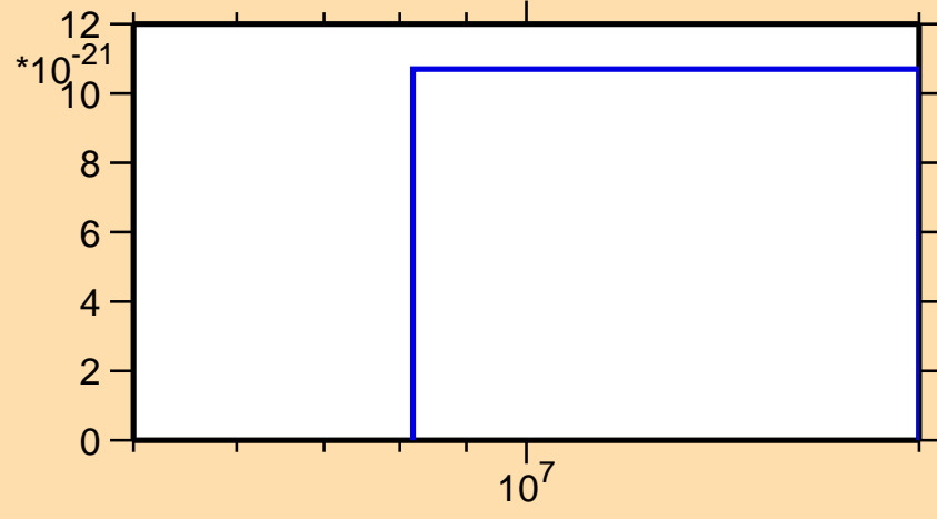
\sigma vs. E for ^{204}\text{Fr}(\text{mt } 42)
