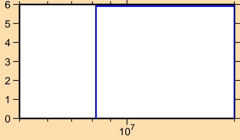
\Delta\sigma/\sigma vs. E for ^{204}\text{Fr}(n,\text{nonel.})
