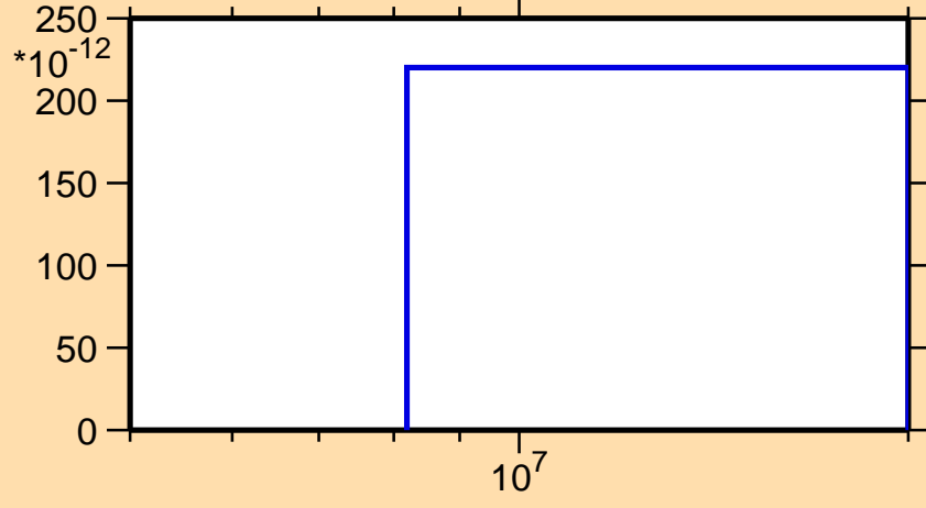
\sigma vs. E for ^{204}\text{Fr}(n,3n\alpha)
