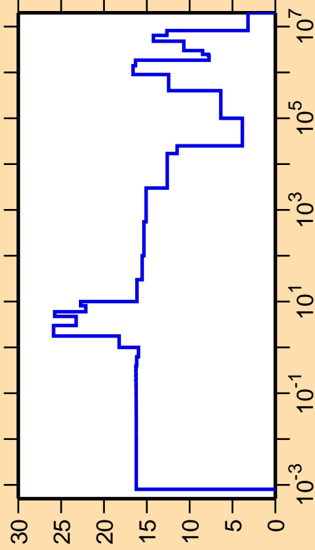
\Delta\sigma/\sigma vs. E for ^{204}\text{Fr}(n,\text{el.})
