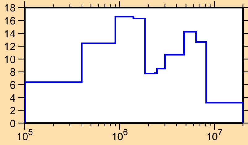
\Delta\sigma/\sigma vs. E for ^{204}\text{Fr}(n, el.)
