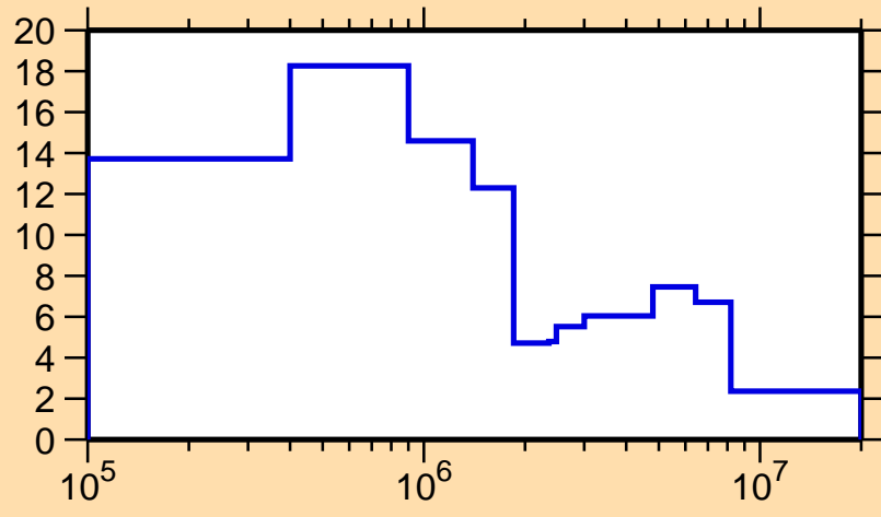
\Delta\sigma/\sigma vs. E for ^{204}\text{Fr}(n,\text{tot.})
