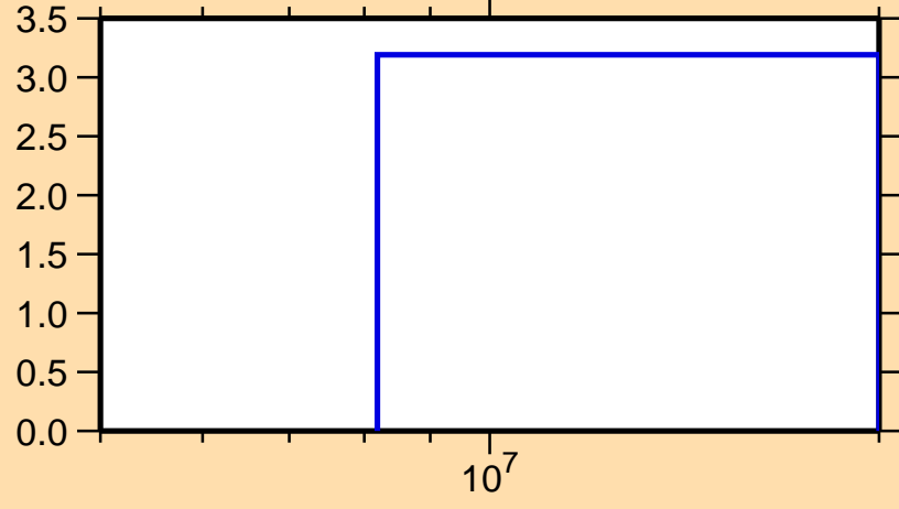
\Delta\sigma/\sigma vs. E for ^{204}\text{Fr}(n,\text{el.})
