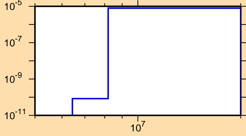
\sigma vs. E for ^{204}\text{Fr}(n,2n\alpha)
