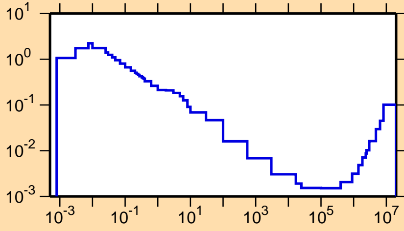
\sigma vs. E for ^{204}\text{Fr}(n,p)
