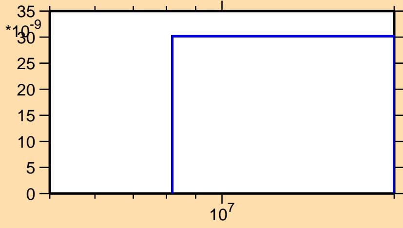
\sigma vs. E for ^{204}\text{Fr}(n,\text{nd})
