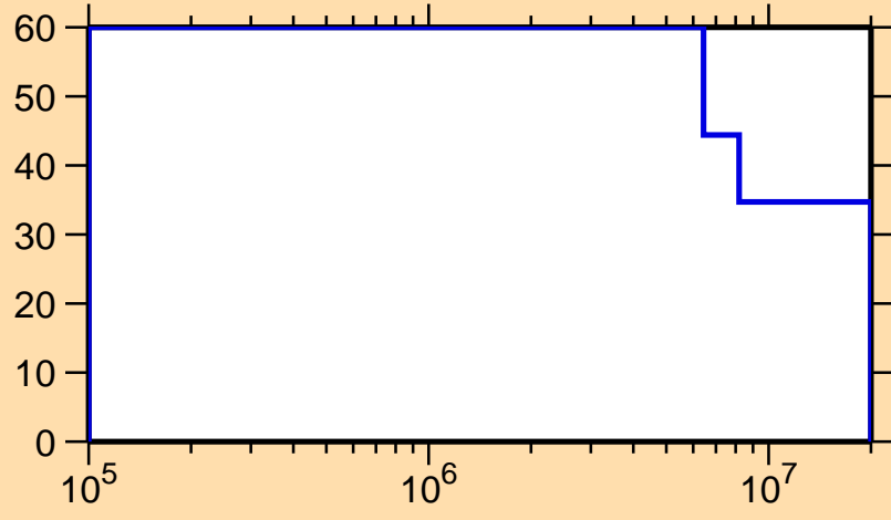
\Delta\sigma/\sigma vs. E for ^{204}\text{Fr}(n,n\text{cont.})
