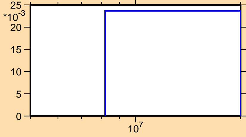
\sigma vs. E for ^{204}\text{Fr}(n,2n)
