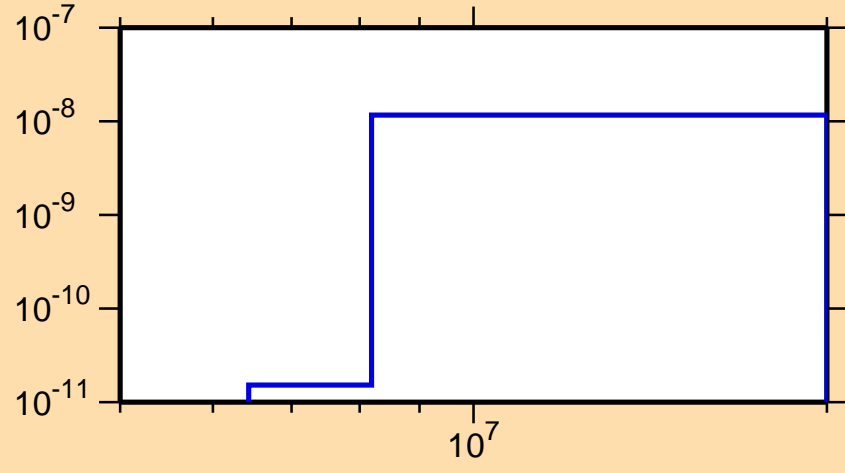
\sigma vs. E for ^{204}\text{Fr}(\text{mt } 45)
