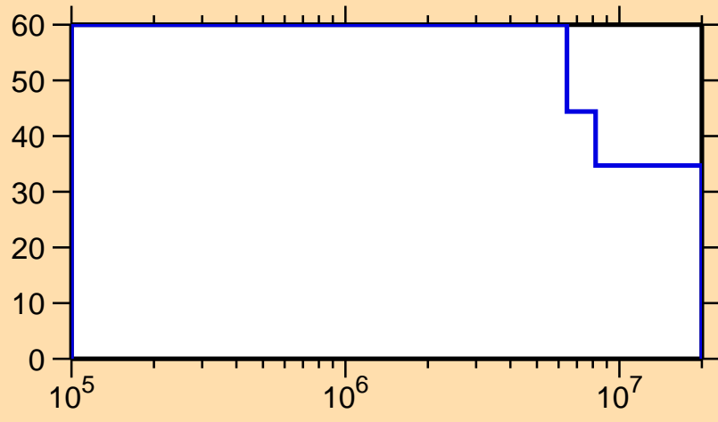
\Delta\sigma/\sigma vs. E for ^{204}\text{Fr}(n,ncont.)
