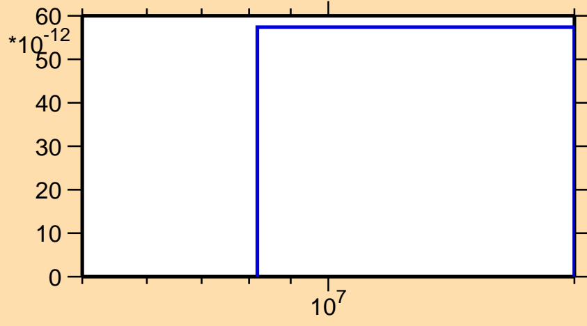
\sigma vs. E for ^{204}\text{Fr}(n,\text{pt})
