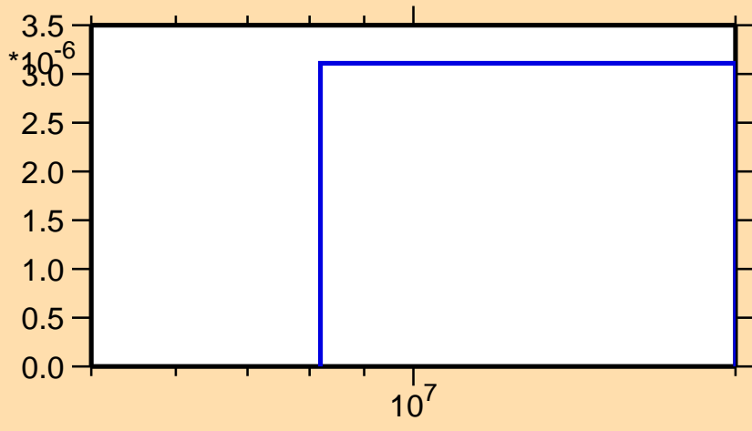
\sigma vs. E for ^{204}\text{Fr}(n,2np)
