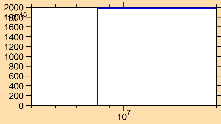
\sigma vs. E for ^{204}\text{Fr}(\text{mt } 34)
