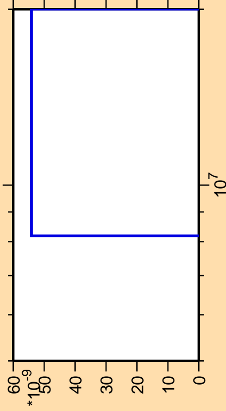
\Delta\sigma/\sigma vs. E for ^{204}\text{Fr}(\text{mt } 42)
