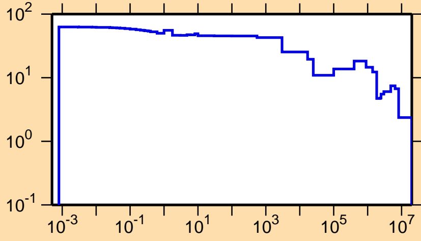
\Delta\sigma/\sigma vs. E for ^{204}\text{Fr}(n,\text{tot.})
