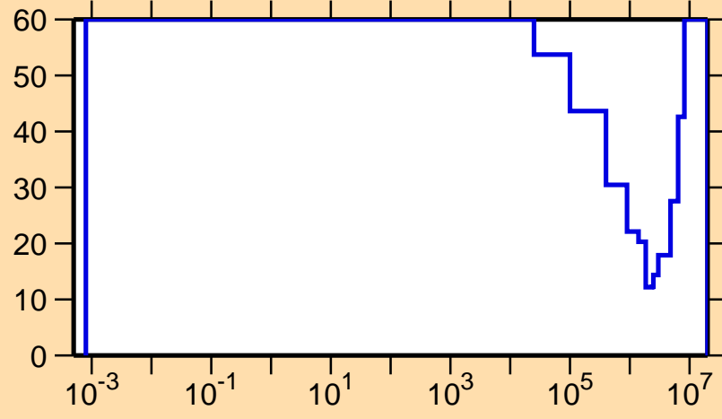
\Delta\sigma/\sigma vs. E for ^{204}\text{Fr}(n,\gamma)
