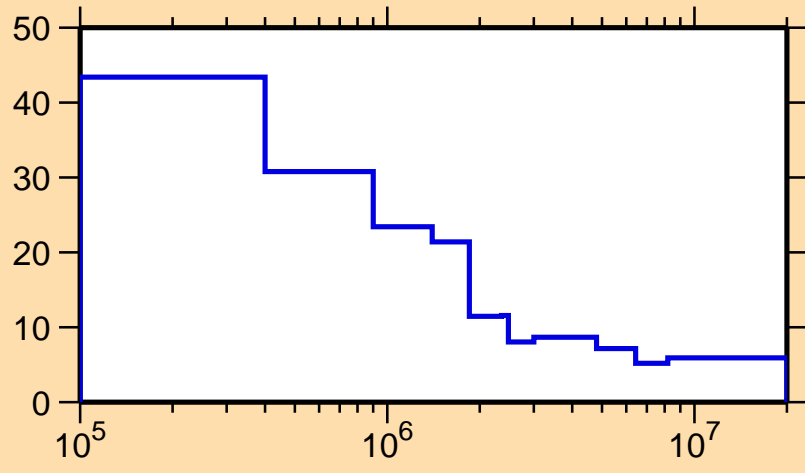
\Delta\sigma/\sigma vs. E for ^{204}\text{Fr}(n,\text{nonel.})
