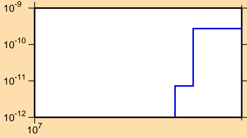
\sigma vs. E for ^{205}\text{Fr}(n,\text{pt})
