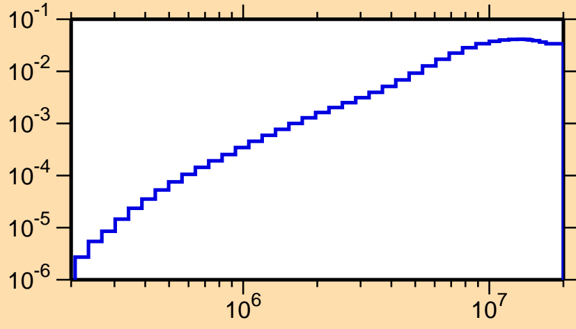
\sigma vs. E for ^{205}\text{Fr}(n,n\alpha)
