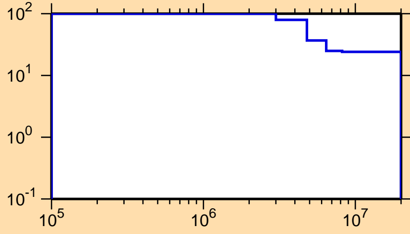
\Delta\sigma/\sigma vs. E for ^{205}\text{Fr}(n,ncont.)
