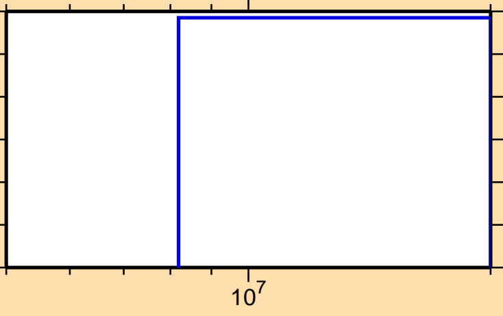
\sigma vs. E for ^{205}\text{Fr}(n,2n)
