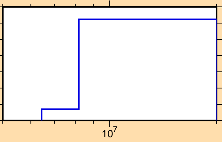
\sigma vs. E for ^{205}\text{Fr}(n,\text{He3})
