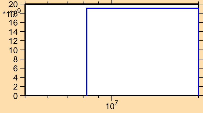
\sigma vs. E for ^{205}\text{Fr}(n,3n\alpha)
