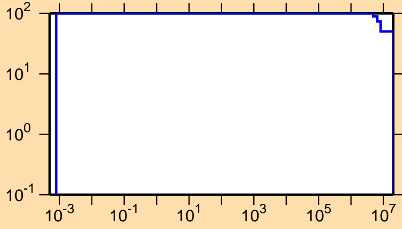
\Delta\sigma/\sigma vs. E for ^{205}\text{Fr}(n,p)
