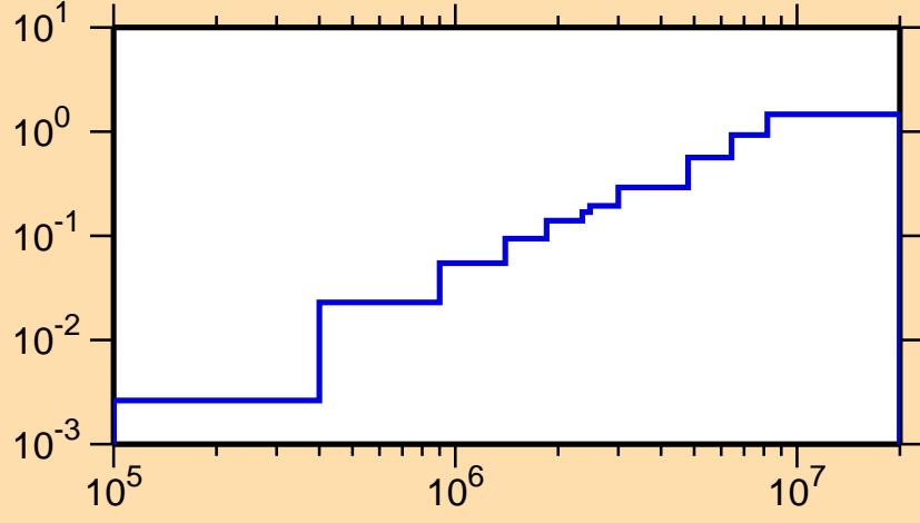
\sigma vs. E for ^{205}\text{Fr}(n,\text{inel.})
