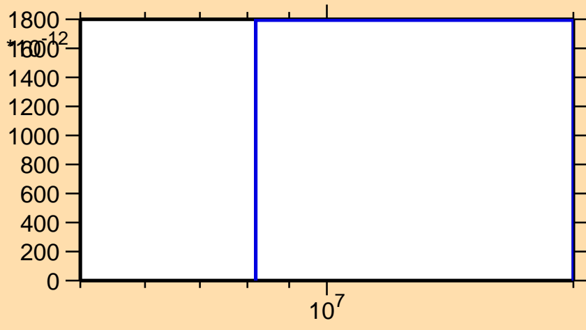
\sigma vs. E for ^{205}\text{Fr}(n,\text{pd})
