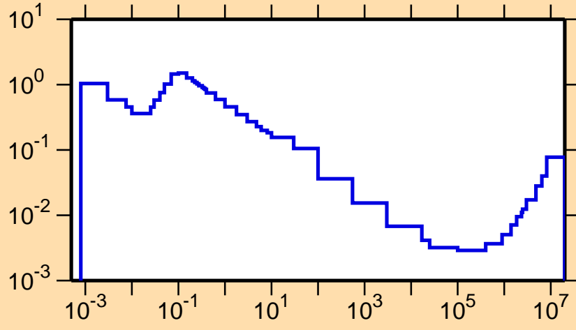
\sigma vs. E for ^{205}\text{Fr}(n,p)
