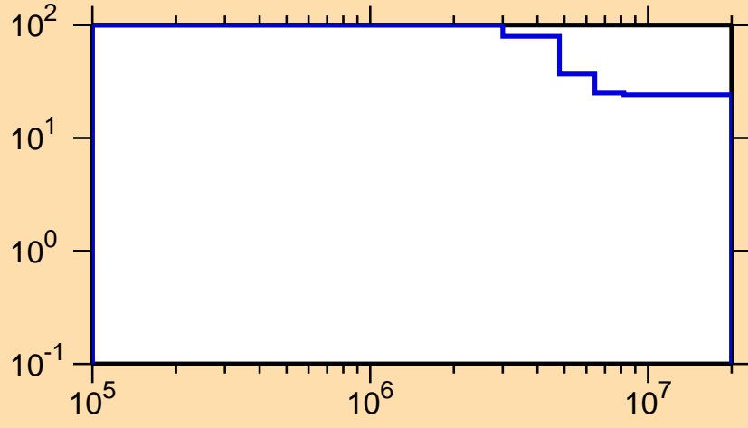
\Delta\sigma/\sigma vs. E for ^{205}\text{Fr}(n,n\text{cont.})
