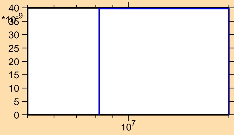
\sigma vs. E for ^{205}\text{Fr}(n,2n\alpha)
