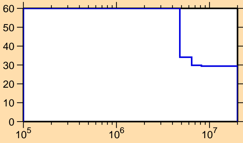
\Delta\sigma/\sigma vs. E for ^{205}\text{Fr}(n,\text{inel.})
