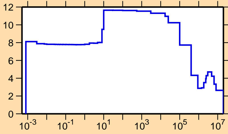
\sigma vs. E for ^{205}\text{Fr}(n,\text{el.})
