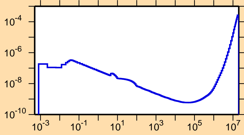
\sigma vs. E for ^{206}\text{Fr}(n,p\alpha)
